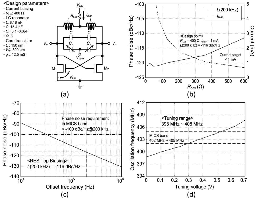
Figure 3. (a) Schematic of LC-VCO with top resistive biasing, (b) phase noise and current consumption in accordance with top resistance, (c) phase noise performance, and (d) tuning range.
