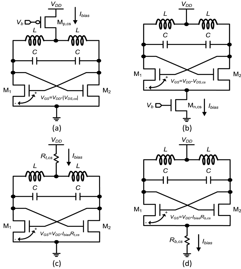
Figure 1. Current biasing techniques of (a) PMOS current source, (b) NMOS current source, (c) top resistive biasing, and (d) bottom resistive biasing.
