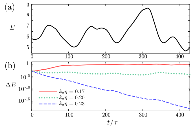
FIG. 1. Continuous data assimilation in the box turbulence. (a) Time series of kinetic energy E(t) in statistically steady states, normalized by the Kolmogorov timescale \tau . (b) Time series of approximation error \Delta E(t) between \mathbf{u}(t) and \tilde{\mathbf{u}}(t) for k_a \eta = 0.17 (solid red), 0.20 (dot green), and 0.23 (dashed blue).
