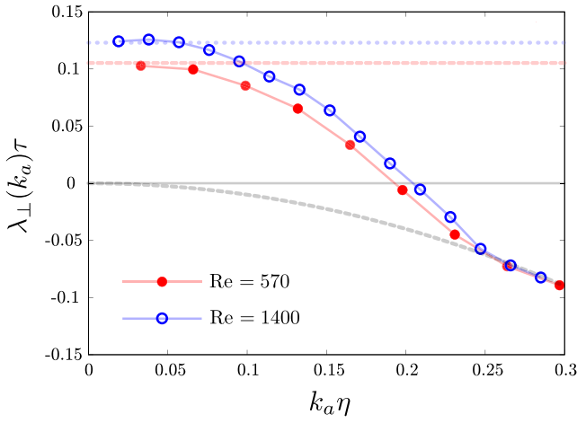
FIG. 3. Reynolds-number dependence of TLEs. The normalization is the same as in Fig. 2. The red solid and blue open circles represent the normalized TLEs for Re = 570 and Re = 1400 , respectively. The horizontal red dashed and blue dotted lines indicate the values of the normalized maximal LEs \lambda\tau for Re = 570 and Re = 1400 , respectively. The gray dashed curve corresponds to \lambda_{\perp}(k_a)\tau = -(k_a\eta)^2 , where the viscous term determines the perturbation dynamics.
