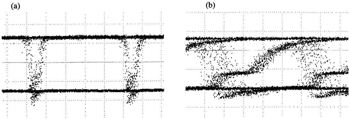
Fig. 6.27: Eye patterns when a serial data stream was transmitted without encoder/decoder. ((a) 100 Mbps/ch, PRBS 2^{11}-1 and (b) 1 Gbps/ch, PRBS 2^{23}-1 )
