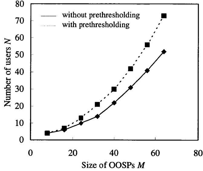
Fig. 2.11: Maximum number of users with the restriction of \text{BER} < 10^{-9} .
