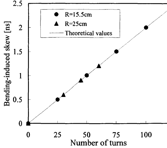
Fig. 3.13: Relation between number of turns and bending-induced skew.
