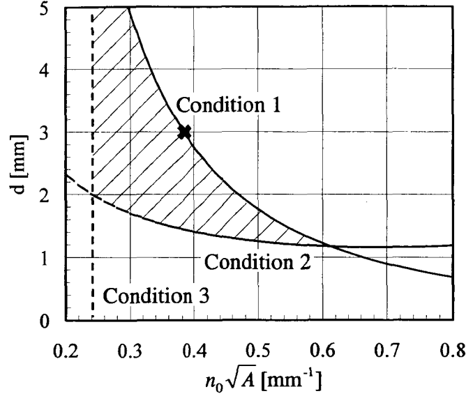
Fig. 4.6: Possible domain of the size of cube BS d and GRIN-rod-lens parameter n_0\text{SQRT}(A) of image fiber couplers which can branch image fibers ( \text{NA} = 0.2 , D = 1.1 mm).
