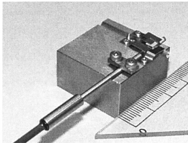
Fig. 6.23: Photograph showing the lens system in the receiver with an image fiber.
