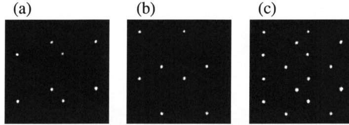
Fig. 6.31: 2 \times 2 optical signals encoded by (a) OOSP 1 and (b) OOSP 2 after propagation through 1-m-long image fibers. (c) Encoded and multiplexed optical signals.
