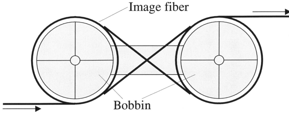
Fig. 3.14: 8-shaped bobbin for winding without increasing skew.
