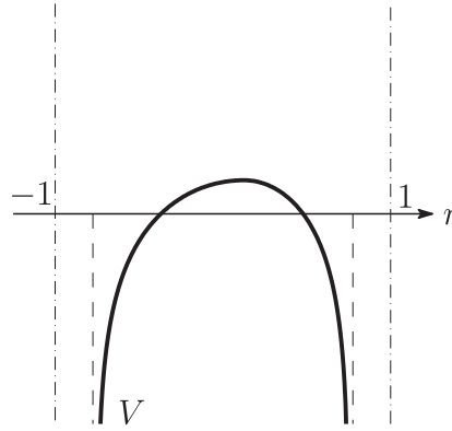
Fig.1.1. The graph of V (Type I)
