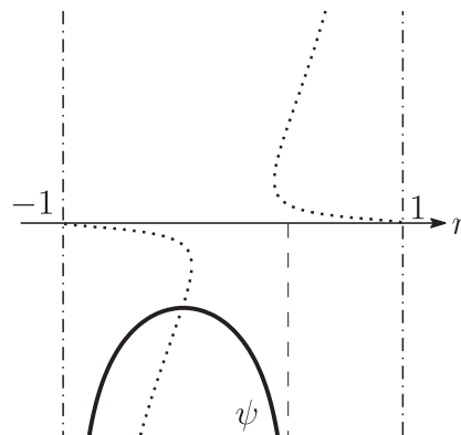
Fig. 2.8. The graph of \psi (Type III)
