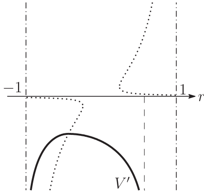
Fig. 2.16. The graph of V' (Type III')
