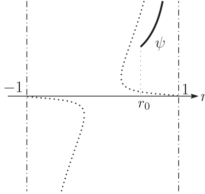
Fig.2.3. The behavior of the graph of \psi in Lemma 2.6
