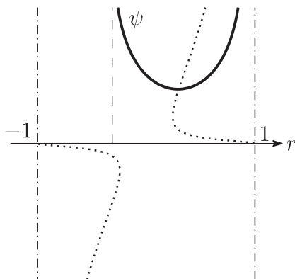
Fig. 2.7. The graph of \psi (Type II)
