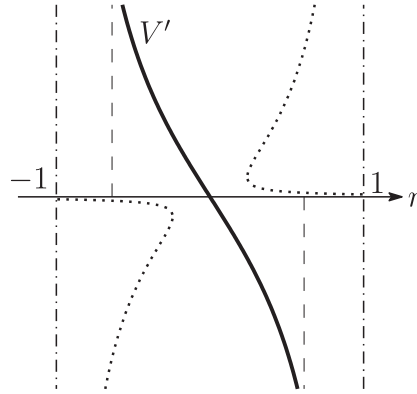
Fig.2.11. The graph of V' (Type I)
