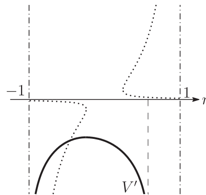
Fig. 2.15. The graph of V' (Type III)
