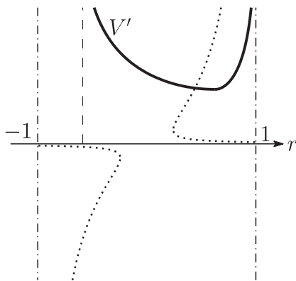
Fig. 2.14. The graph of V' (Type II'')
