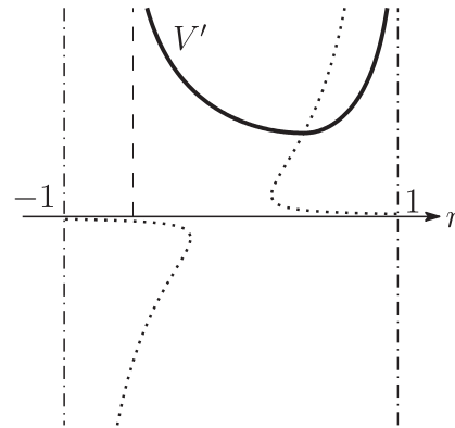
Fig. 2.13. The graph of V' (Type II')
