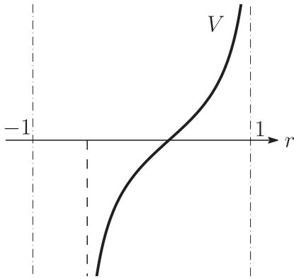
Fig. 1.2. The graph of V (Type II)
