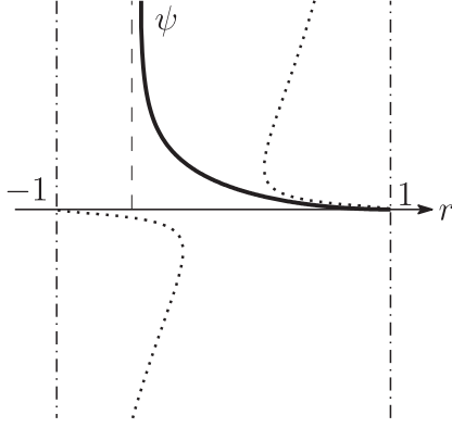
Fig. 2.9. The graph of \psi (Type IV)
