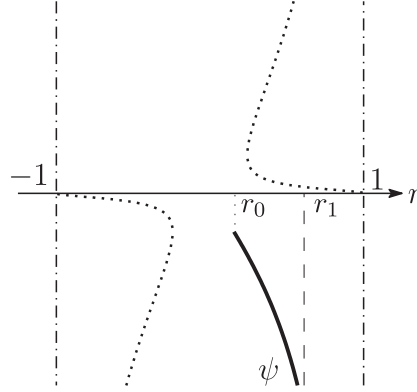
Fig.2.2. The behavior of the graph of \psi in Lemma 2.5
