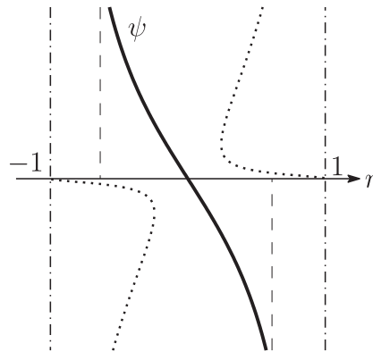
Fig.2.6. The graph of \psi (Type I)
