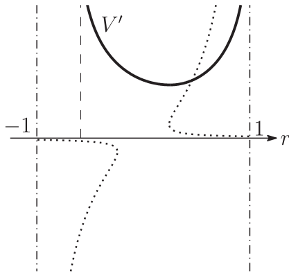
Fig. 2.12. The graph of V' (Type II)
