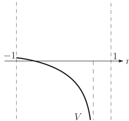
Fig. 1.5. The graph of V (Type V)
