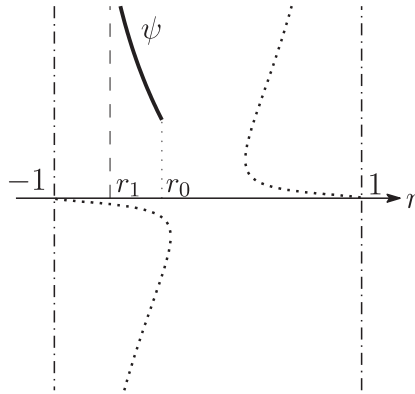
Fig.2.4. The behavior of the graph of \psi in Lemma 2.7
