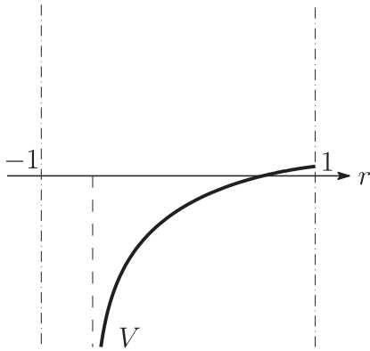
Fig. 1.4. The graph of V (Type IV)
