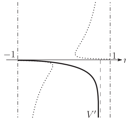
Fig. 2.19. The graph of V' (Type V)
