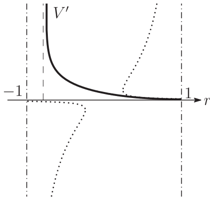
Fig. 2.18. The graph of V' (Type IV)
