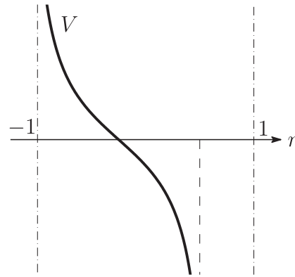
Fig. 1.3. The graph of V (Type III)
