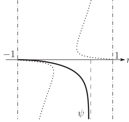
Fig. 2.10. The graph of \psi (Type V)
