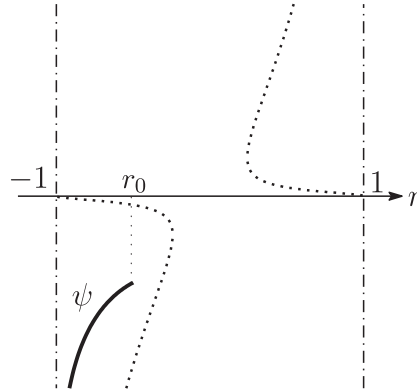
Fig.2.5. The behavior of the graph of \psi in Lemma 2.8
