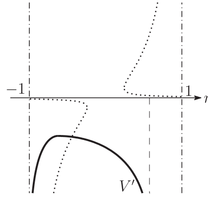
Fig. 2.17. The graph of V' (Type III'')
