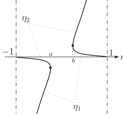
Fig. 2.1. The graph of \eta_1 and \eta_2
