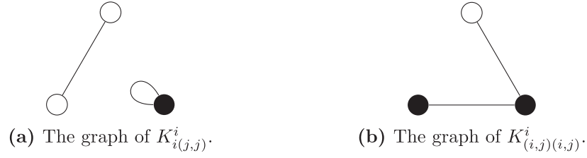
Fig.2. Examples of coefficients which are equal to zero.
