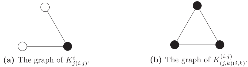
Fig. 1. Examples of non-zero coefficients.
