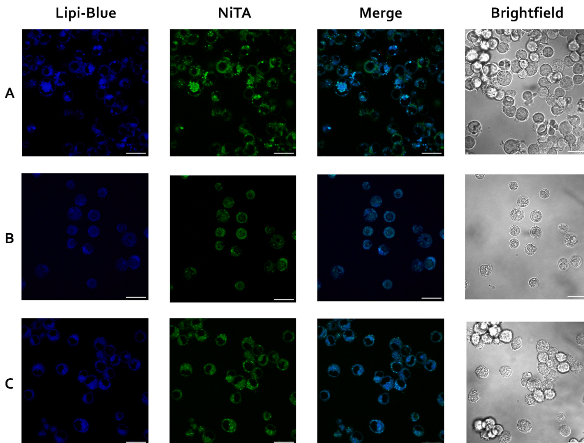
Fig. 2. Live-cell imaging with co-staining of Lipi-Blue and NiTA demonstrates the colocalization of lipid droplets in different cell types. The Pearson correlation coefficient confirms the ability of NiTA to target lipid droplets, with the following results: (A) Jurkat cells: r = 0.79 ; (B) LK35.2 cells: r = 0.83 ; (C) RAW 264.7 cells: r = 0.95 . Jurkat and LK35.2 cells were treated with NiTA at a concentration of 2.5 \mu\text{M} , while RAW 264.7 cells were treated with NiTA at 300 nM concentration. All cells were co-stained with Lipi-Blue (1 \mu\text{M} ) and incubated for 30 min. Images were acquired using an excitation wavelength of 405 nm and emission 400–470 nm for Lipi-Blue, and excitation 488 nm with emission 480–560 nm for the NiTA green channel. Scale bar: 20 \mu\text{m} . (For interpretation of the references to color in this figure legend, the reader is referred to the Web version of this article.)
