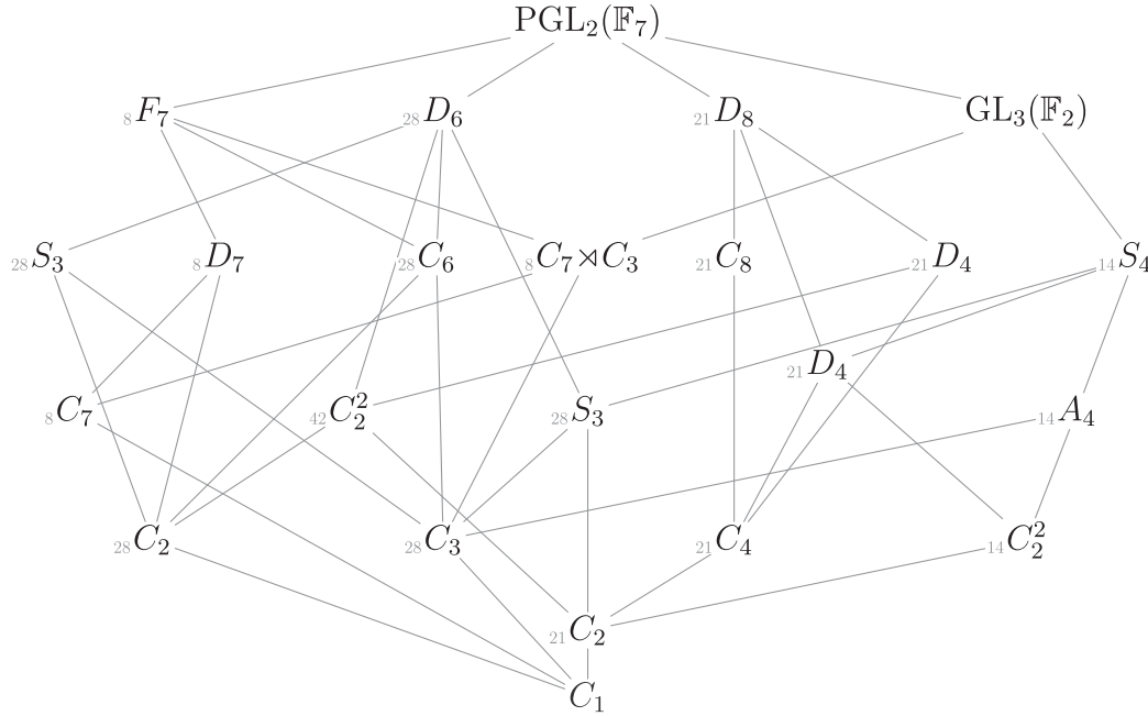
Fig. 1. The lattice of subgroups of \mathrm{PGL}_2(7) .
