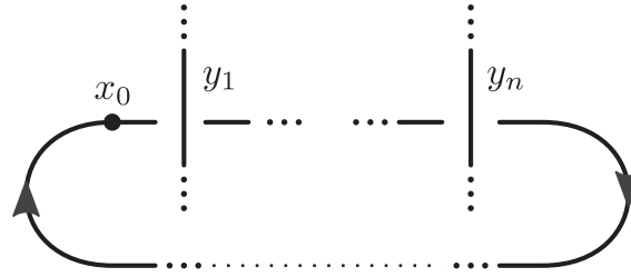
Fig. 1. Definition of \Lambda
