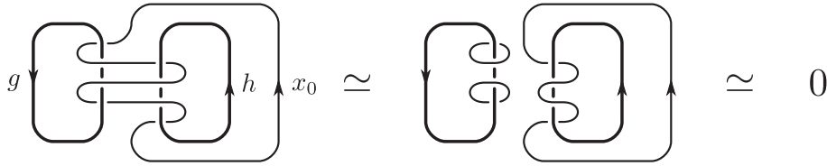
Fig. 3. (D_0, C_0) is null-cobordant
