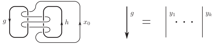
Fig.2. A diagram D_0 with an X -coloring C_0
