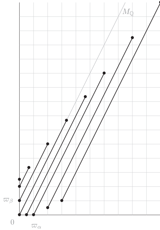
Fig.4. The family (Q^\epsilon)_{\epsilon \geq 0} for \epsilon = 0, \frac{1}{2}, 1, \frac{4}{3}, \frac{5}{3}, 2, \frac{7}{3} and \frac{5}{2} (from right to left).
