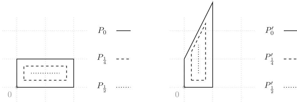
Fig. 1. The families (P_\epsilon) and (P'_\epsilon)
