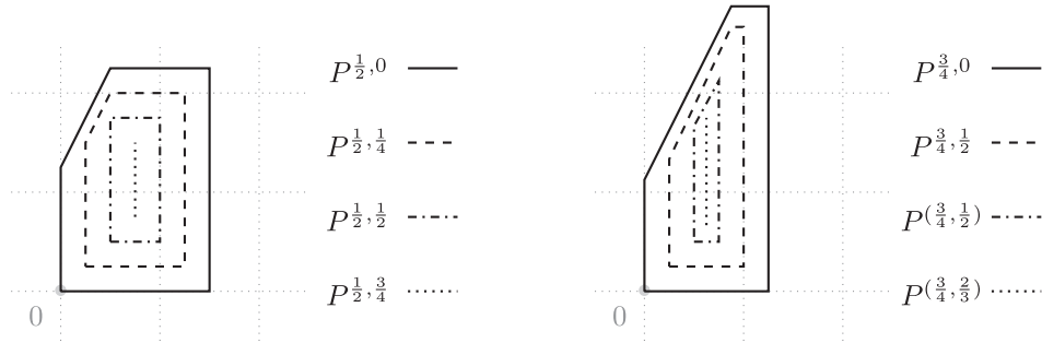
Fig.2. The families (P^{\frac{1}{2},\epsilon}) and (P^{\frac{3}{4},\epsilon})
