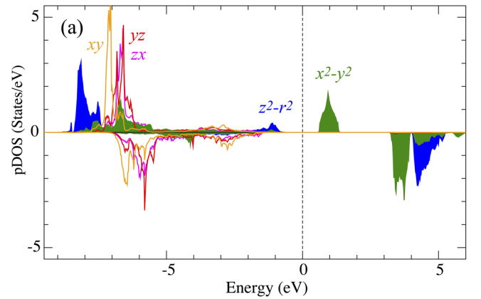
FIG. 3. (a) Projected DOS of the Ni 3d state at the \text{Ni}^{3+} site in 4H structure of \text{H}_{0.5}\text{-SmNiO}_3 using the HSE06 exchange-correlation functional. (b) MLWF contour plot of the occupied Ni e_g state in the \text{Ni}^{3+}\text{O}_2 layer.
