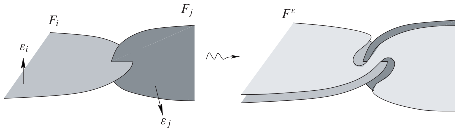
Fig. 3. The surface F^\varepsilon near a clasp; the arrow off F_i indicates the \varepsilon_i -normal direction on F_i in M .
