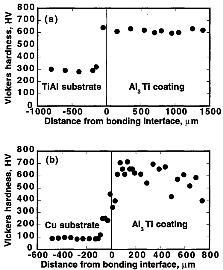
Fig. 2.19 Vickers hardness diprofiles of the Al 3 Ti coating on the (a) TiAl and (b) Cu substrates.
