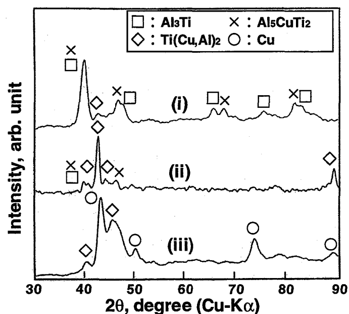
Fig. 3.11 X-ray diffraction patterns of the reaction layers formed at the bonding interface of the \text{Al}_3\text{Ti} coating on the Cu substrate.
