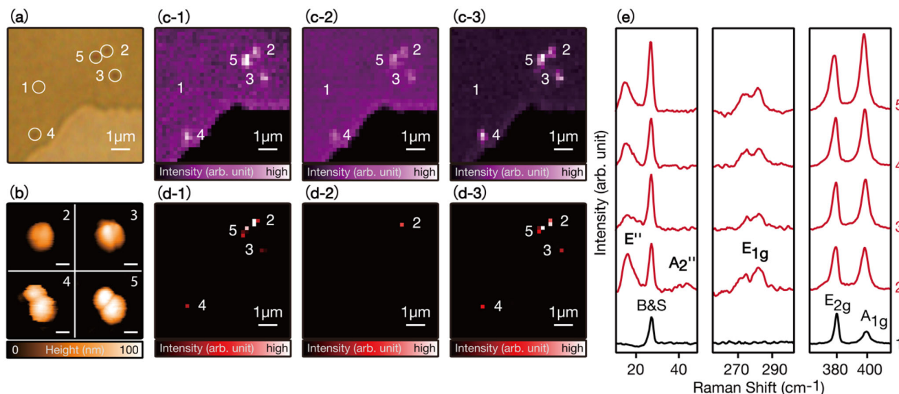
FIGURE 3 | (a) An optical image of a 3-layered MoS 2 sample. (b) A collection of four different AFM images obtained from locations marked from 2 through 5 in (a), showing the existence of silver nanoparticles at these locations. Scale bar: 50 nm. (c-1)–(c-3) Raman intensity images constructed with Raman-active modes: (c-1) shear and breathing modes, (c-2) E 2g mode, and (c-3) A 1g mode. (d-1)–(d-3) Raman intensity images constructed with Raman-forbidden modes: (d-1) E'' mode, (d-2) A 2 '' mode, and (d-3) E 1g mode. (e) Spectra collected at different positions marked in (a). The position marked as 1 corresponds to a region without a silver nanoparticle, and hence shows unenhanced Raman scattering.
