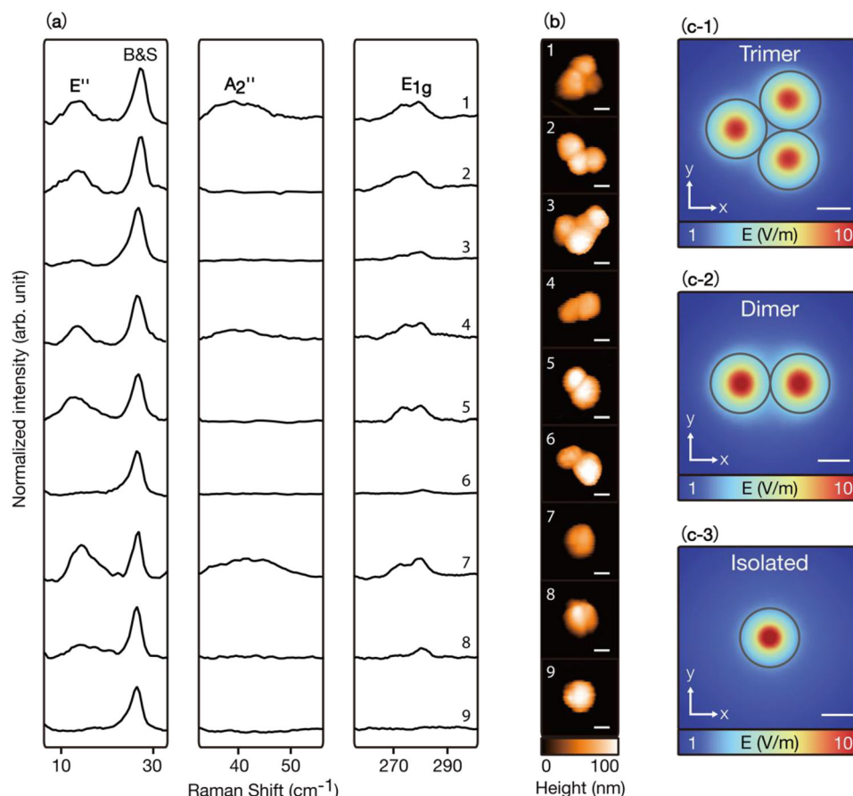
FIGURE 5 | (a) Normalized Raman spectra of a 3-layered MoS 2 sample. (b) AFM images of the corresponding nanoparticles in (a). Scale bar: 50 nm. (c-1), (c-2), (c-3) The electric distributions in the interfacial lateral plane at the contact point between the sample and the nanoparticles of trimer, dimer, and isolated nanoparticle, respectively. Scale bar: 50 nm.
