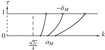
Fig.10. foliation \mathcal{F}_3
