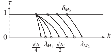
Fig.11. foliation \mathcal{F}_4
