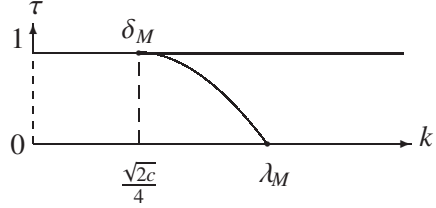
Fig. 6. \lambda_M = \frac{\sqrt{2}c}{4}
