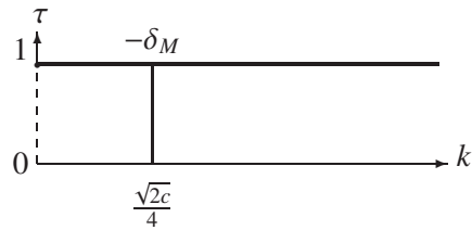
Fig. 2. \lambda_M = \frac{\sqrt{2c}}{4}
