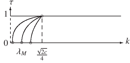
Fig.9. foliation \mathcal{F}_1
