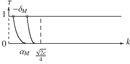
Fig.8. foliation \mathcal{F}_0
