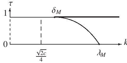
Fig. 7. \lambda_M > \frac{\sqrt{2}c}{4}
