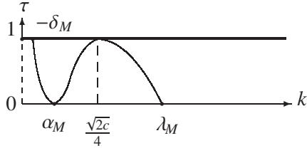
Fig. 3. \frac{\sqrt{2}c}{4} < \lambda_M < \frac{\sqrt{c}}{2}
