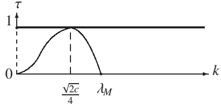
Fig. 4. \lambda_M = \frac{\sqrt{c}}{2}
