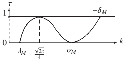
Fig. 1. \lambda_M < \frac{\sqrt{2c}}{4}
