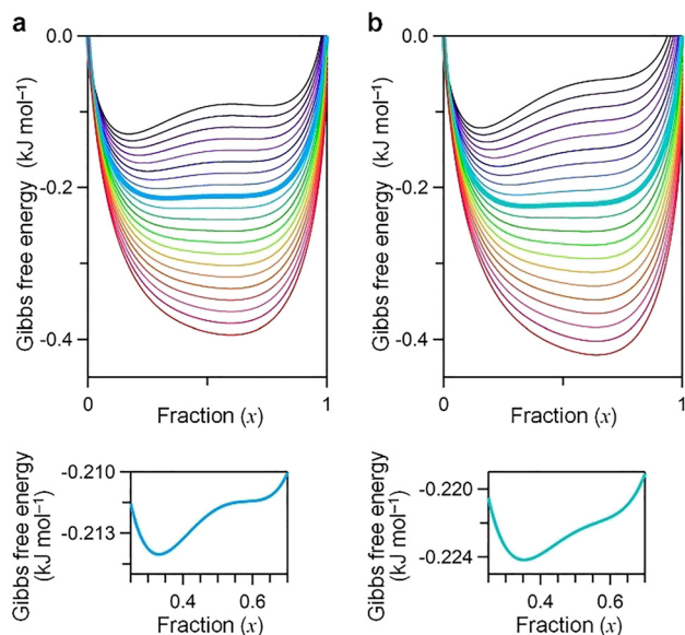
Fig. 6 Temperature-dependent Gibbs free energy ( G ) versus metallic-phase fraction ( x ) curves between the charge-delocalized and charge-localized phases for (a) 1 and (b) 2 , calculated using the Slichter-Drickamer mean-field model at 2 K intervals from 170 K to 130 K (upper panels). Enlarged views around the phase transition region are shown in the lower panel. The curve for 1 corresponds to 146 K, and that for 2 to 148 K. The thermodynamic parameters used were: \Delta H_{\text{trans}} = 500 \text{ J mol}^{-1} , \Delta S_{\text{trans}} = 3.36 \text{ J K}^{-1} \text{ mol}^{-1} , and \gamma = 2500 \text{ J mol}^{-1} for 1 ; and \Delta H_{\text{trans}} = 850 \text{ J mol}^{-1} , \Delta S_{\text{trans}} = 5.67 \text{ J K}^{-1} \text{ mol}^{-1} , and \gamma = 2500 \text{ J mol}^{-1} for 2 . The transition fraction of 1 is 60% of that of 2 . In the calculation, \Delta H_{\text{trans}} was set to 500 \text{ J mol}^{-1} for 1 , which corresponds to the transition enthalpy value assuming the same fraction of transition as in 2 .
