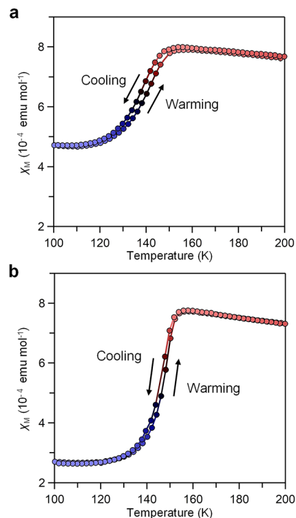
Fig. 4 \chi_M versus temperature plot per mole of \text{Ti}_4\text{O}_7 for (a) 1 and (b) 2 , measured under an external magnetic field of 5000 Oe with a temperature sweep rate of \pm 1.0 \text{ K min}^{-1} .
