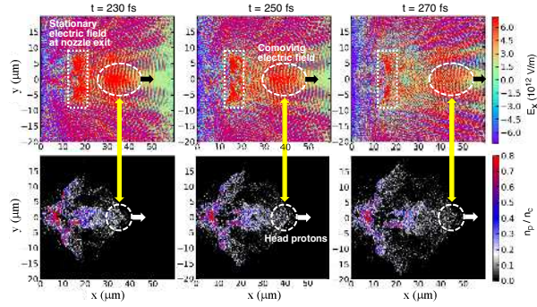
Fig. 3. Upper row: 2D profiles of the longitudinal electric fields E_x . Lower row: proton density profiles at different times, t = 230, 250 , and 270 fs for the MNA target, which correspond to the early times of the afterburner phase; n_c denotes the critical density. The head protons are observed to be continuously accelerated by the comoving electric field. Applied laser and target conditions are the same as in Fig. 2.
