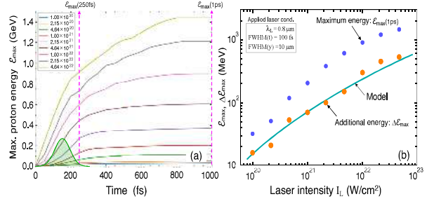
Fig. 5. (a) Temporal evolution of the maximum proton energies at different peak laser intensities (the upper-left inset in units of \text{W}/\text{cm}^2 ). The green Gaussian profile denotes the laser pulse. The time, t = 250 fs, is taken here as the beginning of the afterburner phase. (b) Maximum proton energies at the end, \epsilon_{\text{max}}(1 \text{ ps}) (blue circles), and the additional energies gained in the afterburner phase, \Delta\epsilon_{\text{max}} = \epsilon_{\text{max}}(1 \text{ ps}) - \epsilon_{\text{max}}(250 \text{ fs}) (orange circles). The solid curve is obtained by a simple analytical model based on a self-similar analysis.
