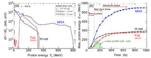
Fig. 2. (a) The proton energy spectra for the MNA, the H-rod, and the foil targets. The H-rod ( 2\text{ }\mu\text{m} -diameter) is just the bullet body taken out from the MNA target, while the foil target is composed of a 1\text{ }\mu\text{m} -thick aluminum with 50\text{ nm} -thick solid hydrogen layer over-coated on the rear surface. (b) The temporal evolution of the three cases of (a). For the MNA target, the maximum proton energy E_{\text{max}} is read to be increasing at the rate of 160\text{ MeV}/100\text{ fs} even after the laser illumination is finished at t \approx 250\text{ fs} .
