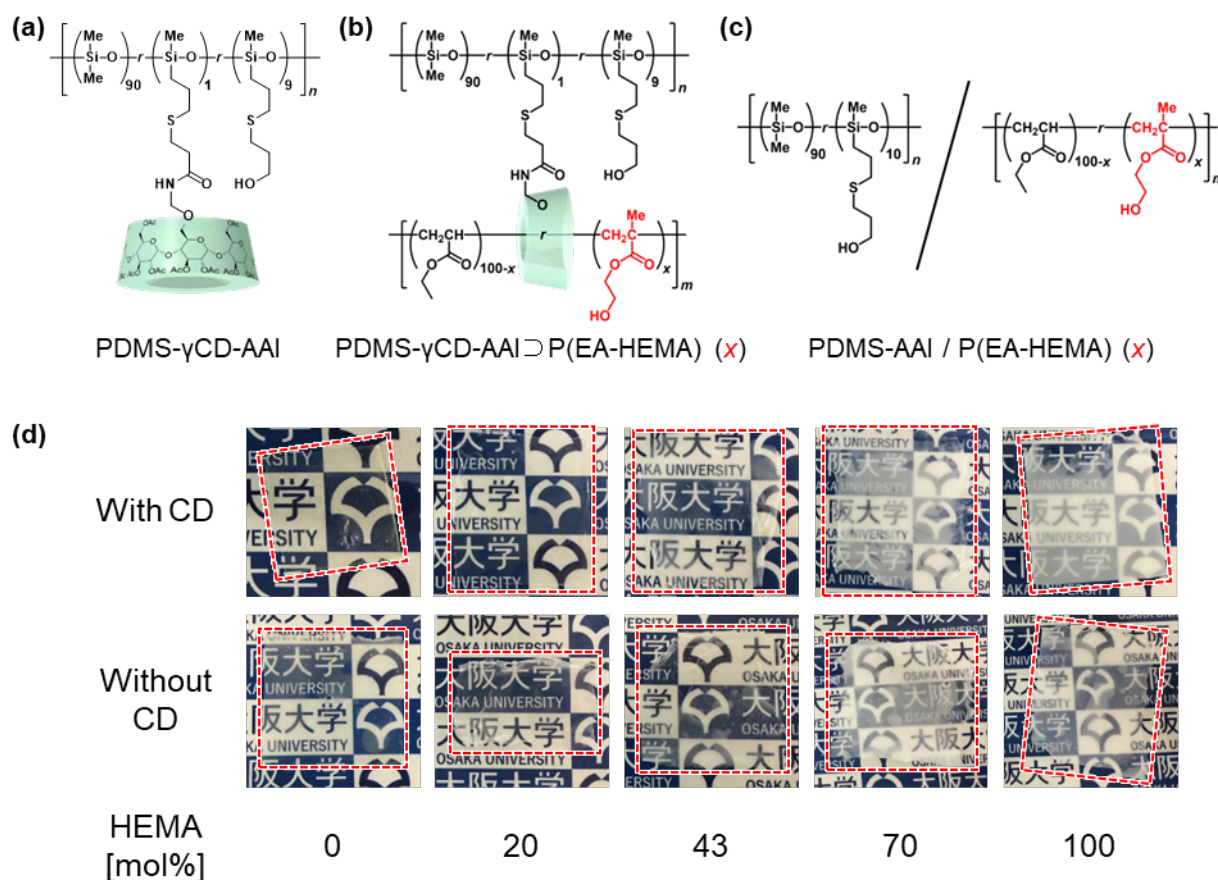
Fig. 2 Chemical structures of (a) PDMS- \gamma CD-AAI, (b) PDMS- \gamma CD-AAI \supset P(EA-HEMA) ( x ), and (c) PDMS-AAI/P(EA-HEMA) ( x ) blends without movable crosslinks. x is the mol% HEMA content in acrylate copolymers. (d) Photographs of PDMS- \gamma CD-AAI \supset P(EA-HEMA) ( x ) and PDMS-AAI/P(EA-HEMA) ( x ).
