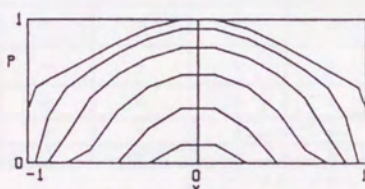
PRESSURE DISTRIBUTION (PROFILE) K=2.600 LAMBDA= .128 PMAX= .1416
