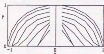
PRESSURE DISTRIBUTION (BODY PLAN) K=2.600 LAMBDA= .128 PMAX= .1416
