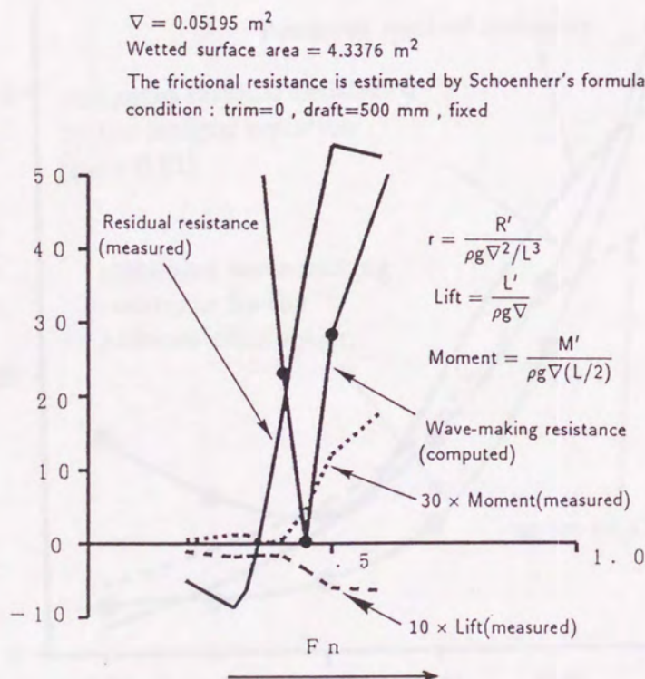
Figure 53 Experimental residual resistance [S 2 ]
