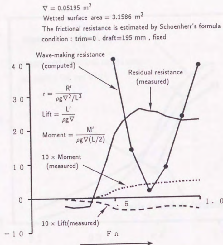
Figure 52 Experimental residual resistance [S 1 ]
