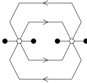
Fig. 9. Immersion for w_C(\Gamma) = 2
