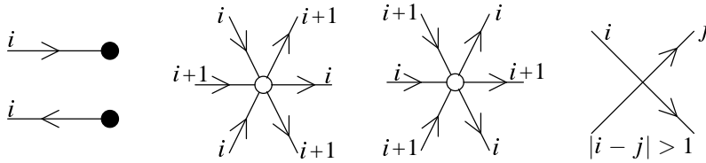
Fig. 1. Vertices and a crossing of a surface braid chart
