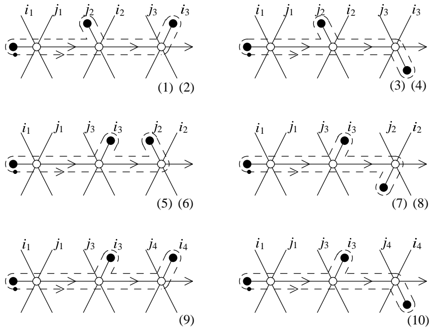
Fig. 12. Rails of length more than three.
