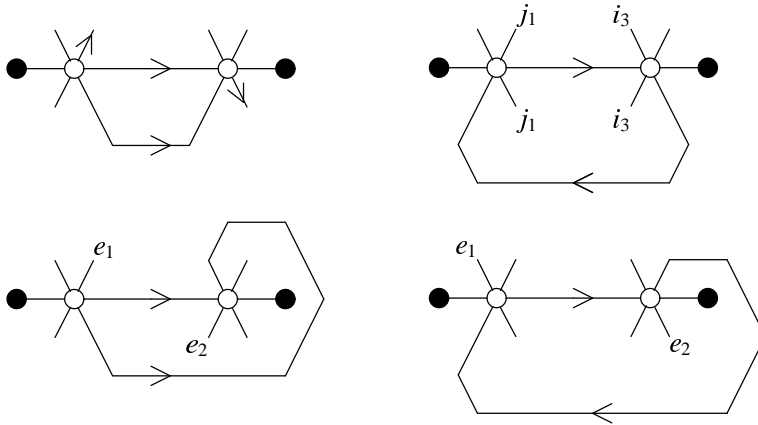
Fig. 14. Two edges incident to W_1 and W_3 .
