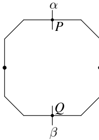
Fig. 4. Pull back of handle rail
