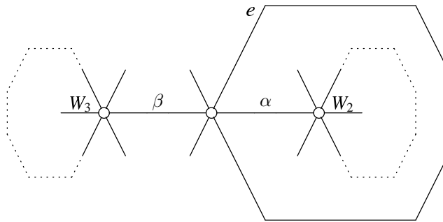
Fig. 11. An edge satisfying \text{init}(e) = \text{term}(e)
