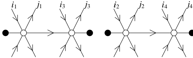
Fig. 13. Two rails of length three.
