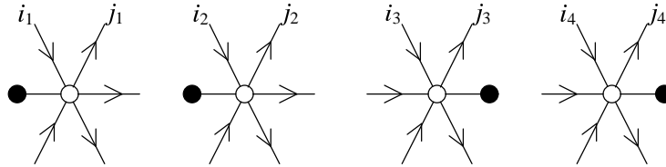
Fig. 10. Labels and orientations of four white vertices.
