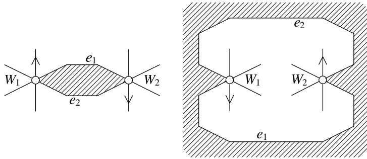
Fig. 6. Canceling pair
