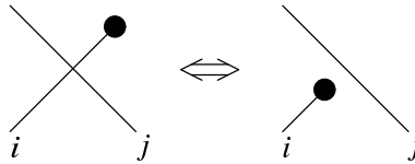
Fig. 2. Chart moves of type II
