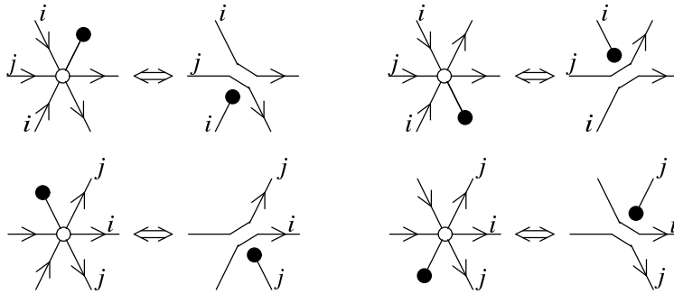
Fig. 3. Chart moves of type III
