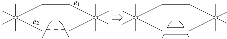
Fig. 8. Delete crossings with arcs in X
