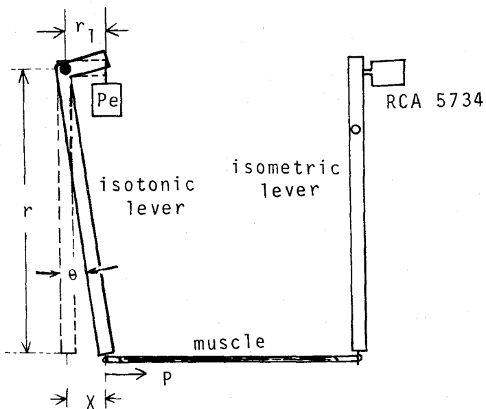
Fig. A-1 Schematic drawing of the employed lever system.
