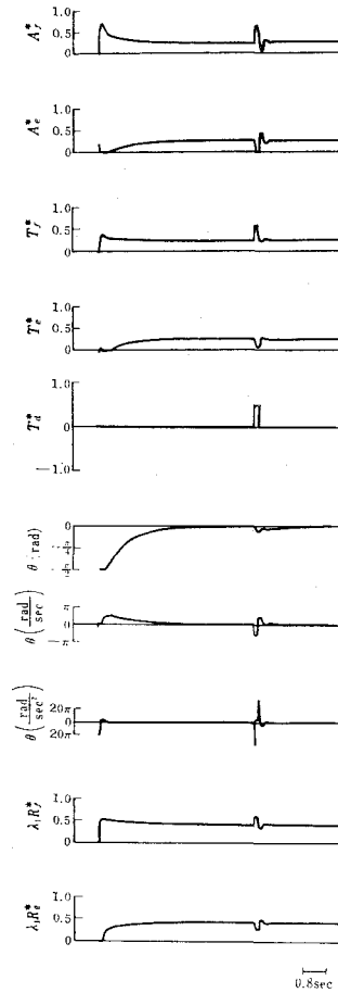
Fig. 5.5 Simulated response of postural control action to show the transient response of flexing movement and response to disturbance torque ( T_d^* ).
