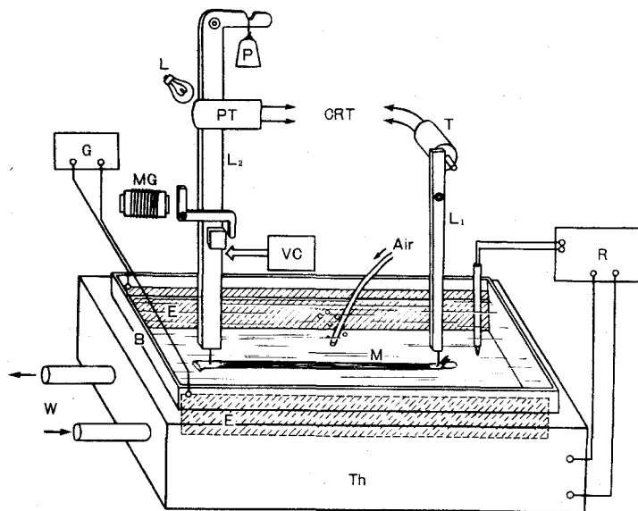
Fig. 2.10 Diagram of the recording system.
