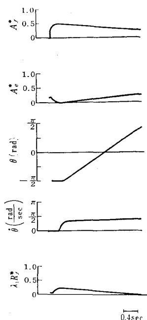
Fig. 5.14 Simulated result to show the possibility of velocity control of flexion movement. Neuronal connection, Fig. 5.13 (B); H_{\alpha}^* = 0.25 , M = 1.0 Kg, \Gamma_f^* = 0.34 , these values satisfy the relation of Eq. (5.16). Spindle GII afferent path, flexor reflex pattern; GII afferent fibers operate always.
