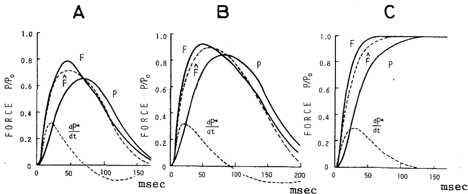
Fig. 4.10 Comparison of the approximate curve ( \hat{F} ) with the active state curve determined by graphical analysis (F). \hat{F} = P + dP^*/dt ; P, measured isometric tension curve; A, single pulse; B, 2 pulses; C, 16-pulse stimulation; stimulus interval, 12.5 msec.
