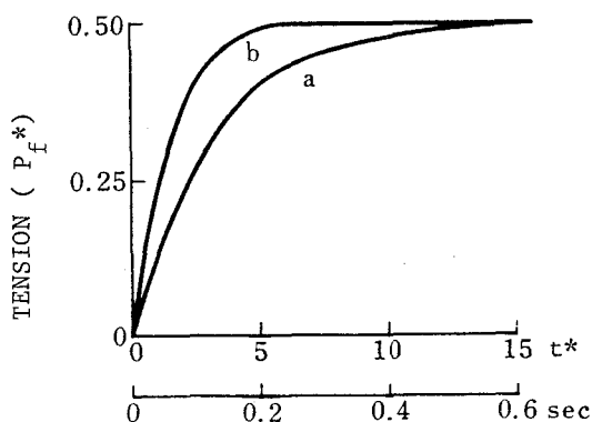
Fig. 5.11 Simulation result to show the effect of Golgi tendon GIb feedback on the tension development to step change in H_{\alpha}^* . Curve a, in the absence of GIb feedback, \delta_1=0 , H_{\alpha}^*=0.5 ; curve b, in the presence of GIb feedback, \delta_1 K_T^* = 1.0 , H_{\alpha}^* = 1.0 .
