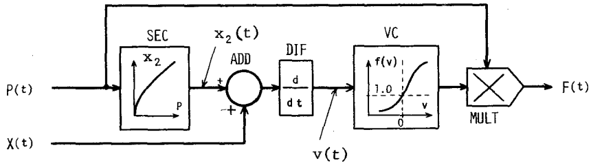
Fig. 4.3 Blockdiagram for computer calculation of the active state curve F(t), from tension curve P(t) and shortening curve X(t). SEC, function element generating the tension-extension (P-x 2 ) relation of SEC, (input, P; output, x 2 ); VC, function element generating the v - f(v) relation of VC, (input, v; output, f(v)); ADD, adder; DIF, differentiator; MULT, multiplier.
