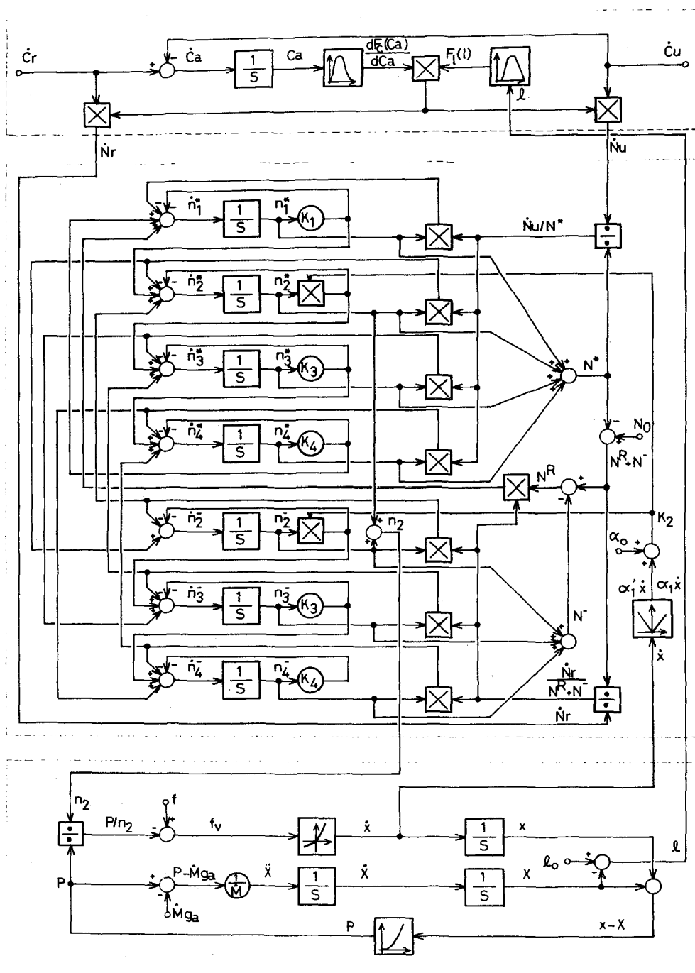
Fig. 6.5 Mathematical model of muscle contraction programmed on a computer.
