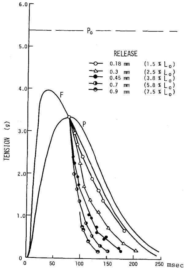
Fig. 4.13 Effect of the amount of quick release on the falling phase of the active state during isometric twitch. Amount of release is shown in the figure. P, Tension curve; F, active state curve determined by graphical analysis; P_0=5.4 gwt; L_0=12 mm; 10^\circ\text{C} .
