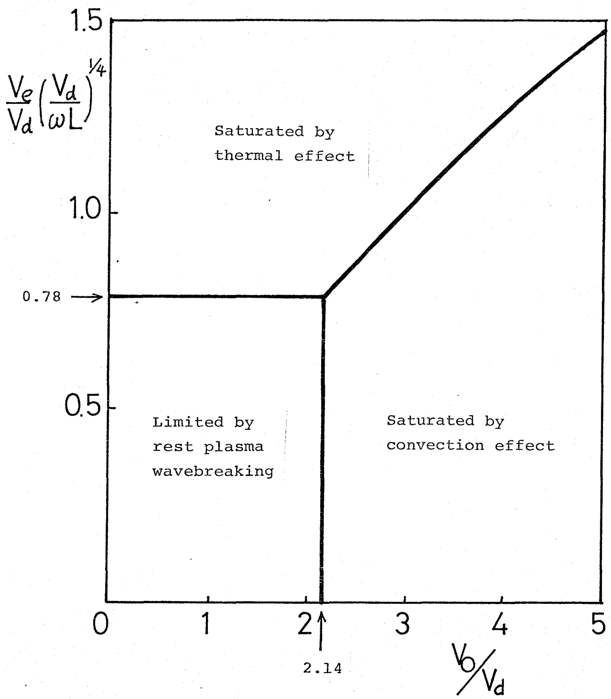
Fig. 5.6 Diagram for the competition between the effect of rest plasma wavebreaking, the thermal effect, and the convection effect.
