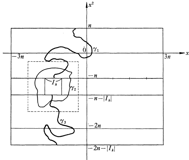
Fig. 3 event H_{n,k}
