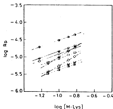
Fig. 57. Dependence of the rate of polymerization on the monomer concentration at 50°C: [I], 4 \times 10^{-8} mol/l. —: APS; pH, (○) 2.20; (●) 6.80; (◆) 10.40. ---: AIBN; pH, (□) 2.10; (■) 6.90; (■) 10.00. ---: SMP; pH, (◇) 8.40; (◆) 9.10.
