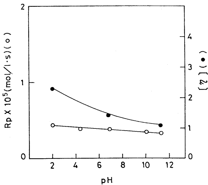
Fig. 45. Dependence of the rate of polymerization and [\eta] of polymer on pH of polymerization medium at 50°C. [M-Glu], 0.2 mol/l; [AIBN], 4 \times 10^{-3} \text{ mol/l} .
