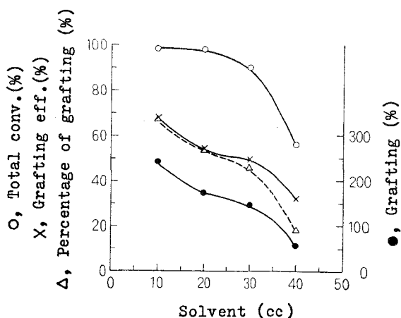
Fig. 79. Effect of amount of solvent. [NR], 0.01 mol; [M-Glu], 0.01 mol; [BPO], 3.3 mmol/l; 80°C; 4 hr; Solvent, Toluene : Dioxane = 2 : 1.
