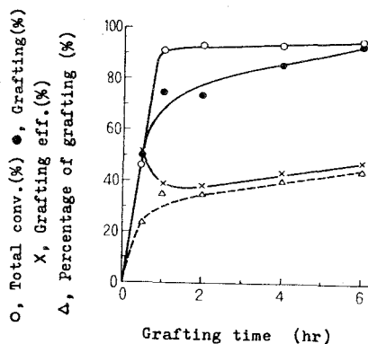
Fig. 90. Effect of grafting time.
