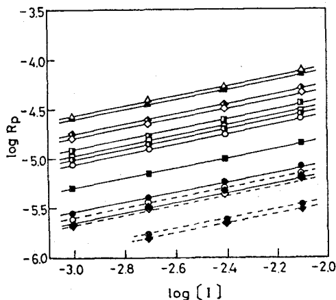
Fig. 43. Dependence of the rate of polymerization on the initiator concentration at 50°C: [Monomer], 0.1 mol/l; —, APS; ---, AIBN. Symbols are the same as in Fig. 42
