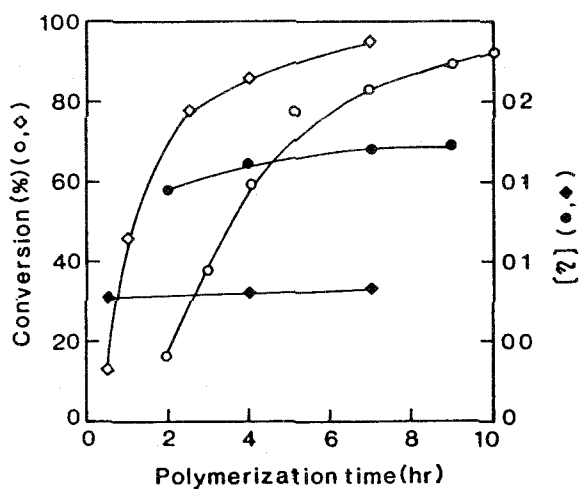
Fig. 6. Effect of polymerization time on polymerization in dioxane at 60°C or 80°C. [M-Gly], 1.4 mol/l; [BPO], 4.13 \times 10^{-3} mol/l. ○, ●, 60°C; ◇, ◆, 80°C.
