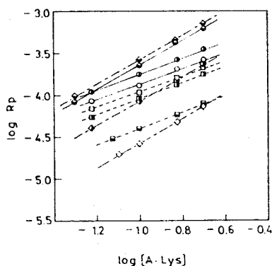
Fig. 56. Dependence of the rate of polymerization on the monomer concentration at 50°C: [I], 4 \times 10^{-8} mol/l. —: APS; pH, (○) 2.10; (●) 6.40; (▼) 9.10. ---: AIBN; pH, (□) 2.30; (■) 6.40; (■) 7.40. ---: SMP; pH, (◇) 6.50; (◆) 7.20; (◆) 9.10.
