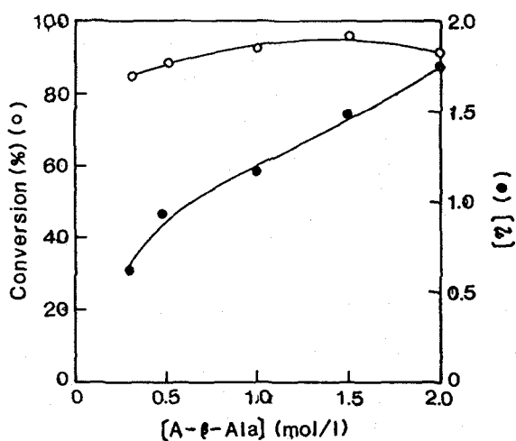
Fig. 14. Effect of the monomer concentration on polymerization in dioxane at 60°C.
