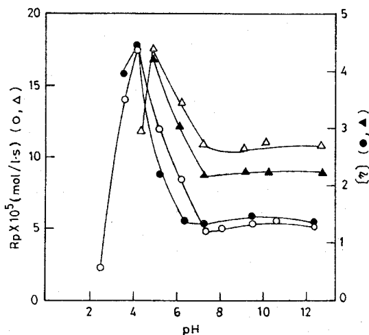
Fig. 35. Dependence of the rate of polymerization and [\eta] of polymer on pH of polymerization medium at 50°C:
