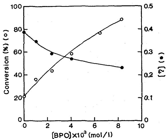
Fig. 13. Effect of amount of BPO on polymerization in dioxane at 60°C.
