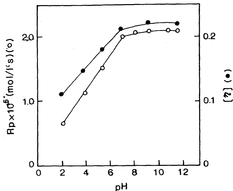
Fig. 27. Dependence of the rate of polymerization and [\eta] of polymer on pH of polymerization medium at 50°C:
