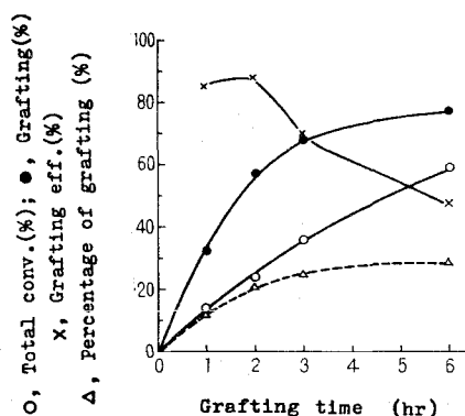
Fig. 94. Effect of grafting time.
