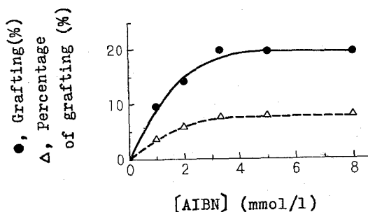
Fig. 95. Effect of concentration of AIBN
