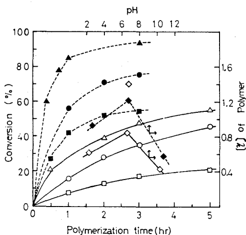
Fig. 46. Aqueous polymerization of N -(2-diethylaminoethyl)acrylamide (I) and methacrylamide (II) with APS. [Monomer] : 1.0 mol/l, [APS] : 1.0 \times 10^{-2} mol/l. Polymerization temp. : 60°C — : Polymerization of I, ..... : Polymerization of II Initial pH = ○ : 2.20, △ : 7.00, □ : 10.55, ● : 2.96, ▲ : 6.95, ■ : 10.80 ◇, ◆ : [\eta] (Polymerization time : 3 hr)
