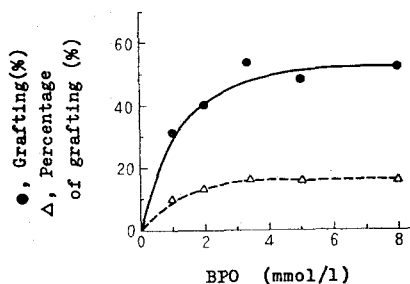
Fig. 96. Effect of concentration of BPO
