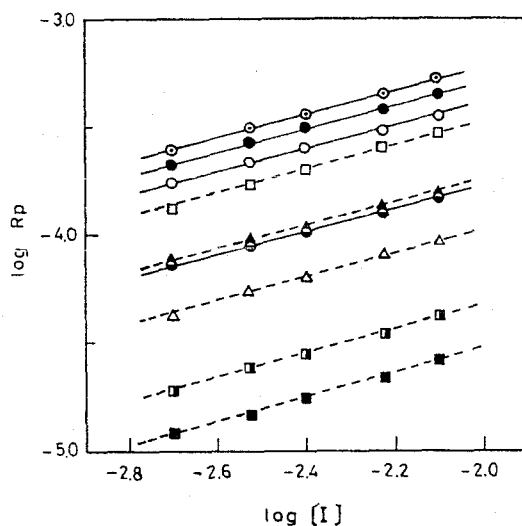
Fig. 26. Dependence of the rate of polymerization on the initiator concentration at 50°C: [A-Gly], 0.2 mol/l.
