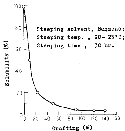
Fig. 76. Relation between solubility and grafting. Steeping solvent, Benzene; Steeping temp., 20-25°C; Steeping time, 30 hr.
