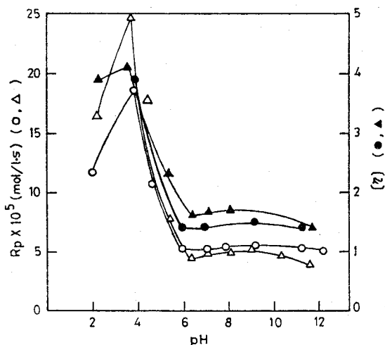
Fig. 34. Dependence of the rate of polymerization and [\eta] of polymer on pH of polymerization medium at 50°C:
