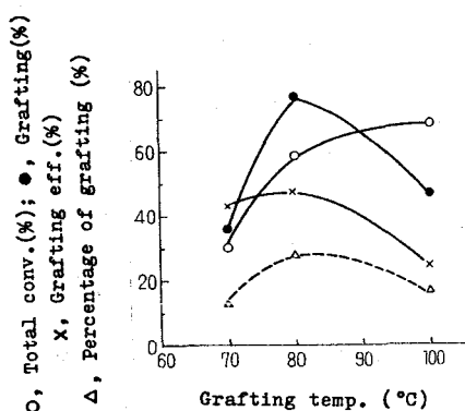
Fig. 93. Effect of grafting temperature.
