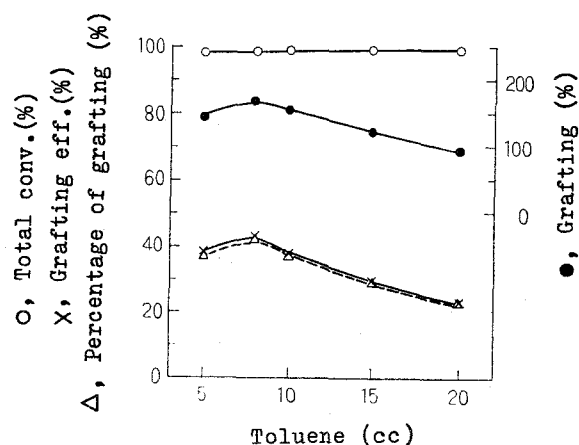
Fig. 83. Effect of amount of solvent.
