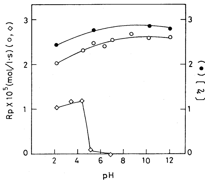
Fig. 44. Dependence of the rate of polymerization and [\eta] of polymer on pH of polymerization medium at 50°C. [APS], 4 \times 10^{-3} \text{ mol/l} ; ○ and ●, [M-Glu], 0.2 mol/l; ◇, [M-Glu], 0.1 mol/l.
