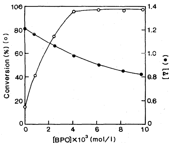
Fig. 1. Effect of amount of BPO on polymerization in dioxane at 60°C. [A-Gly], 1.0 mol/l; Polymerization time, 1hr.
