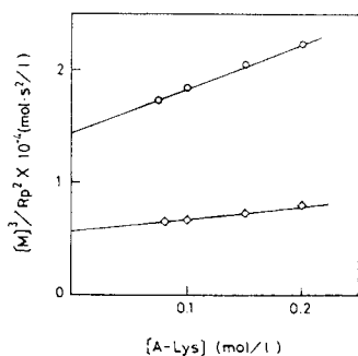
Fig. 60. Plot of [M]^3/R_p^2 against [M] . [SMP], 4 \times 10^{-3} mol/l; 50^\circ\text{C} ; ( \diamond ), pH 6.50; ( \circ ), pH 9.10.
