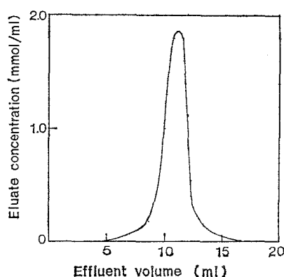
Fig. 98. Elution curve of \text{Cu}^{2+} with 2N-HCl.
