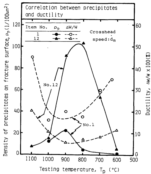
Fig. 9 Density of precipitates and ductility vs. temperature.
