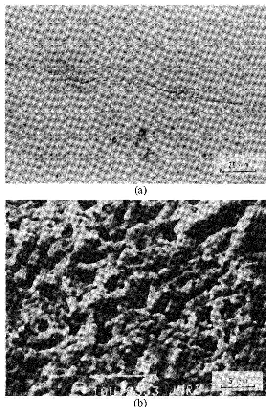
Fig. 1 Features of migrated grain-boundary (a) and intergranular fracture surface (b) after actual weld cracking test for Item No. 10.
