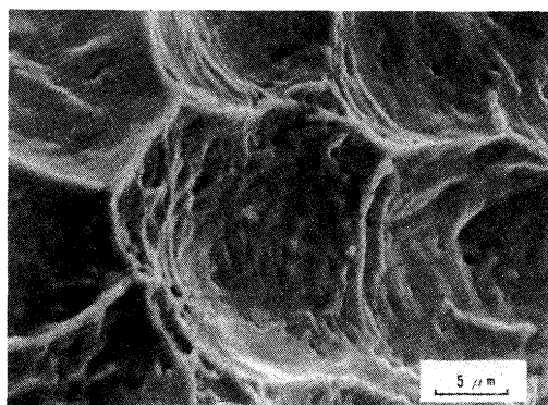
Fig. 13 An example of intergranular dimple including several precipitates, Item No. 1, 900°C.
