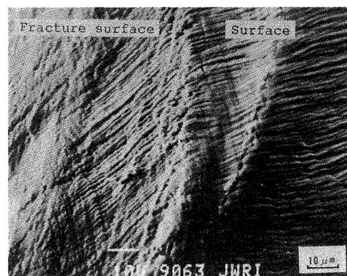
Fig. 14 Correlation between slip bands on specimen surface and feature of intergranular fracture surface in Item No. 12 (900°C, \dot{d}_h )
