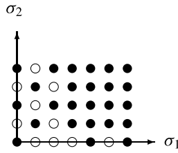
Fig. 1. The semigroup \mathbb{N}A in Example 6.15
