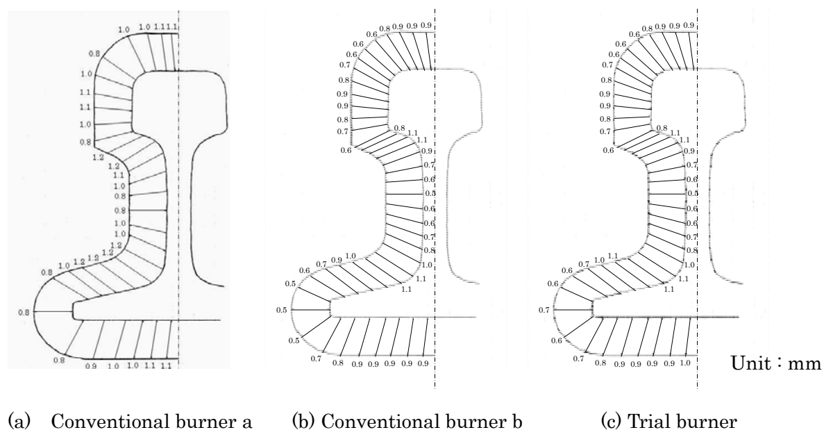
Fig.5-3 Tip arrangement and diameter of each burner
