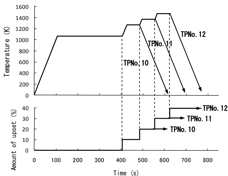
Fig.3-12 Joining conditions of TPN0.10-12
