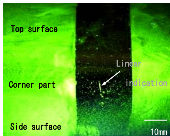
Fig.4-9 The appearance of linear indication in magnetic particle test (1) : TPNo.R-1
