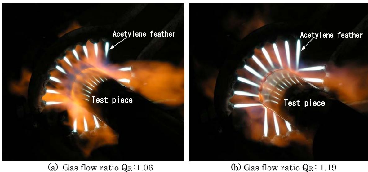
Fig.4-3 The appearance of combustion flame
