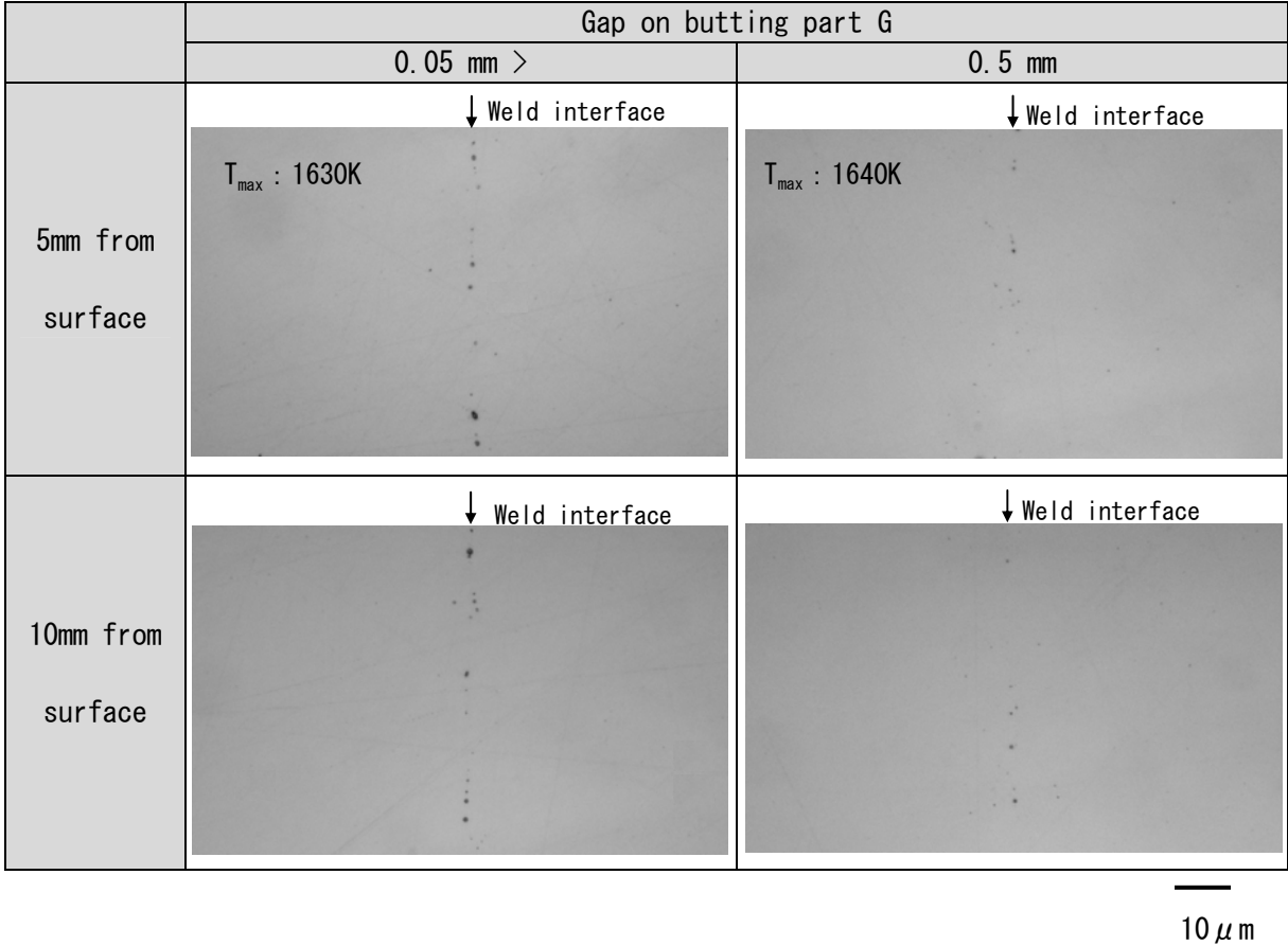
Fig.4-6 The state of oxide inclusions on cross-section (3) Q_R : 1.19 , P : 20\text{MPa}
