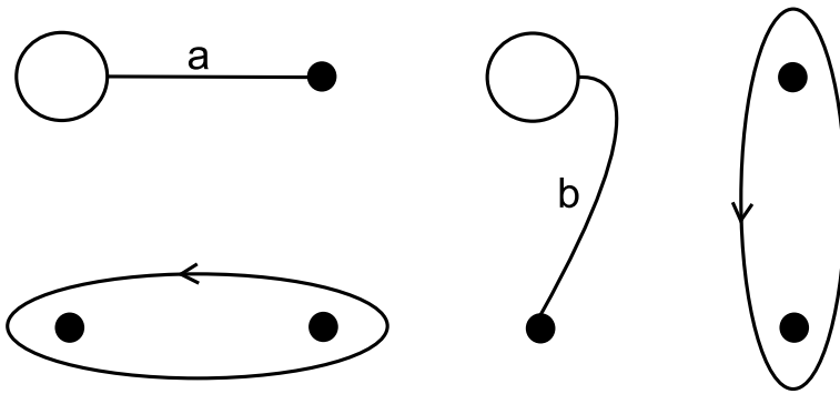
Fig. 3. Curves of Dehn half-twists *a = \sigma_1 and *b = \sigma_2 .
