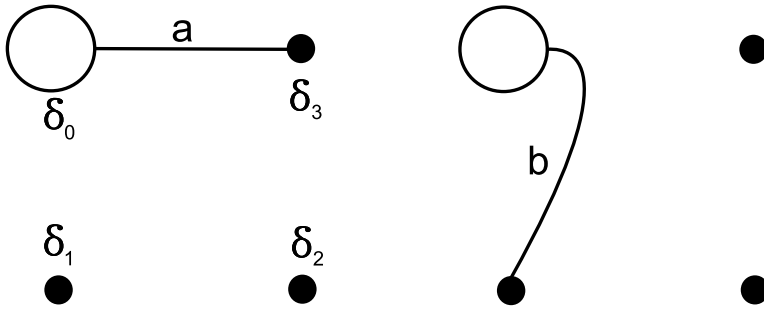
Fig. 2. Generators a and b of the cord quandle \hat{Q} .
