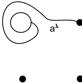
Fig. 4. a^\lambda = a * a^{-4} * b * a * a * b —full twist along \delta_0 of the cord a .
