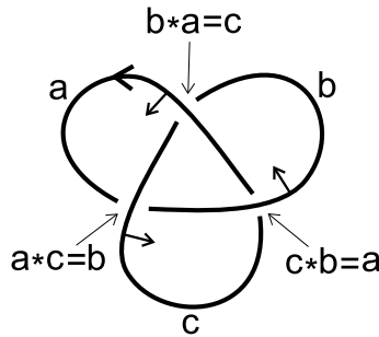
Fig. 1. Generators and relations of the fundamental quandle of the trefoil knot.
