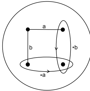
Fig. 5. Generators of “the fundamental quandle of the closed trefoil knot.”
