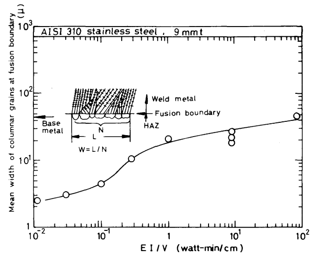
Fig. 2 Variation of Mean Width of Columnar Grains at Fusion Boundary with Welding Heat Input (E·I/V).
