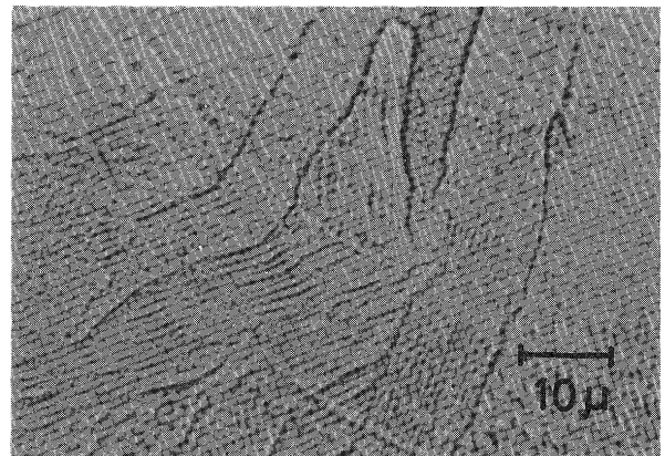
Fig. 8 A Typical Example of Unusual Growth Mode in Cell Structure Observed in Rapidly Solidified Weld Metal.
