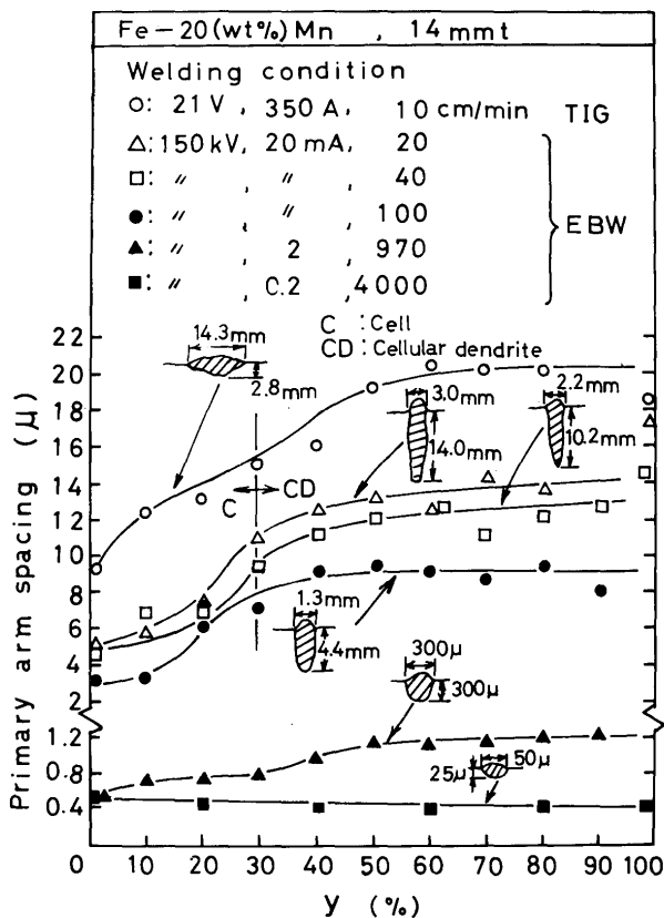
Fig. 6 Variation of Primary Arm Spacing with y (%) in Weld Metal for Fe-20 (wt%) Mn alloy.
