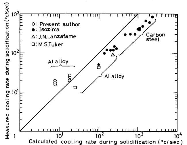
Fig. 1 Comparison of Measured Cooling Rate with Calculated Cooling Rate during Weld Solidification.
