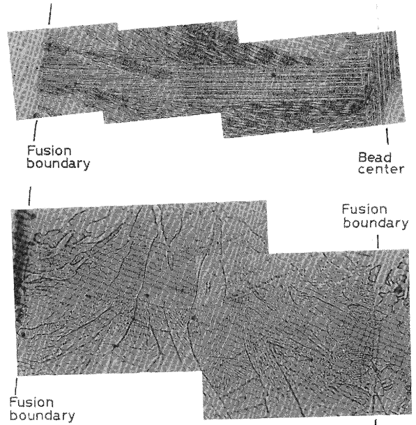
Fig. 7 Structural Changes in Weld Metal of AISI 310 Stainless Steel. (a) TIG Arc Weld, 17V-250A-10cm/min (x42). (b) EBW Weld, 150kV-0.2mA-300cm/min (x600).
