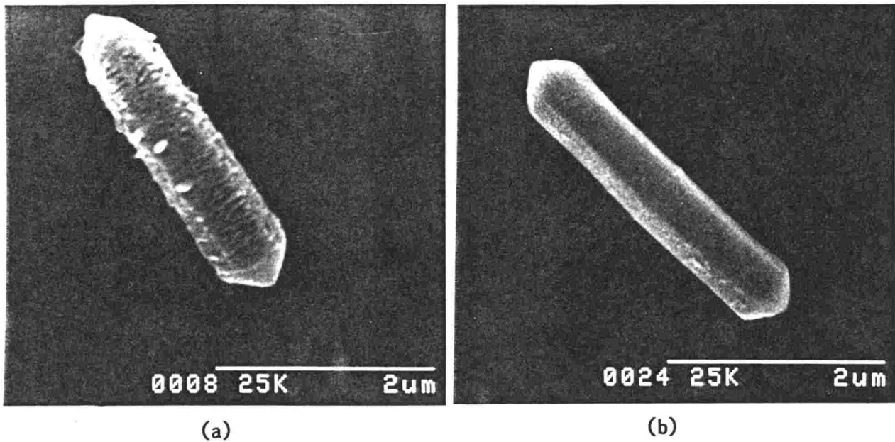
Figure 1-11. Scanning electron micrographs of an incipient crystal (a) prepared in LP at 330°C for 3min (b) washed in 1N-KOH solution.
