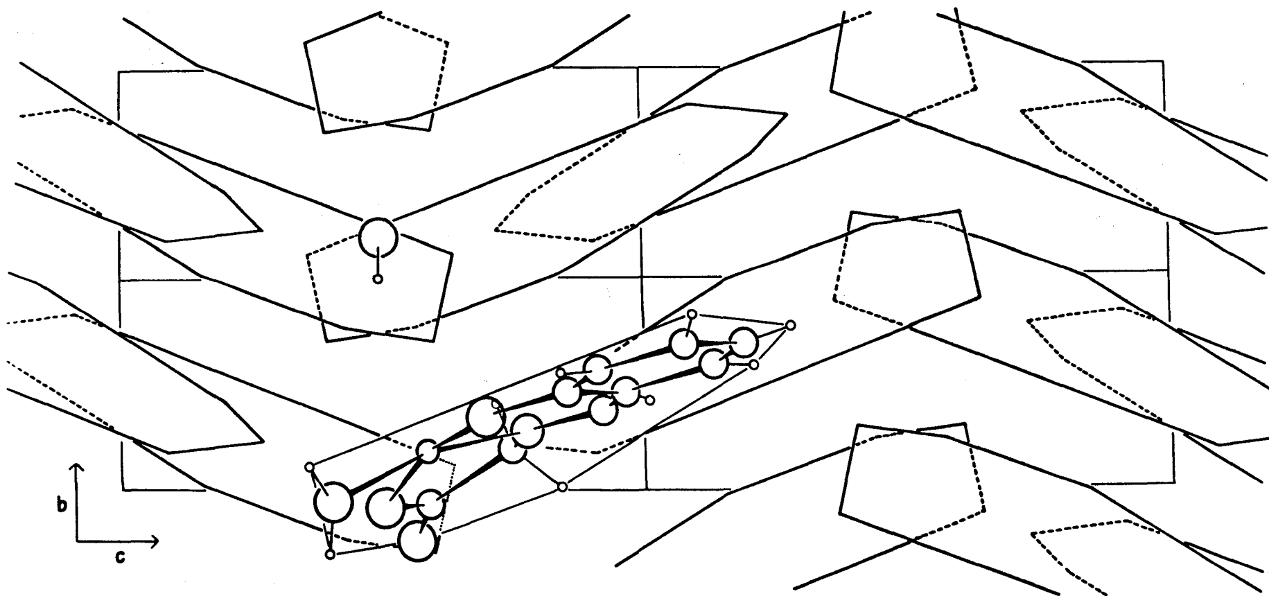
Fig. 11. A schematic Figure of the Crystal Structure of SGCH , looking down along the a axis.
