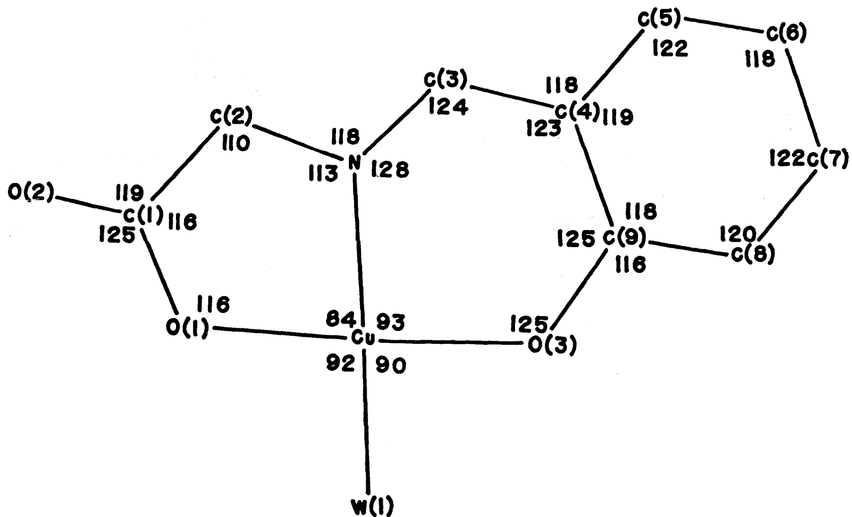
Fig. 4. Bond Angles in the Molecule of SGCT .
