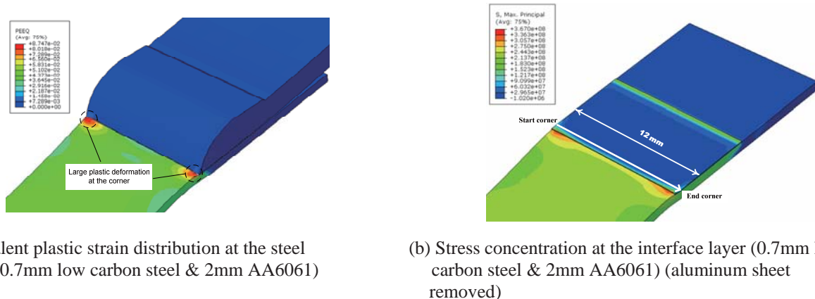
Fig.11 Plastic strain distribution and stress concentration at interface layer corners or edges
