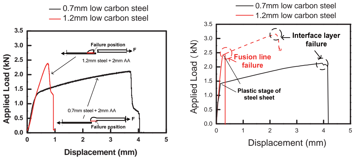
(a) measured L-D curve for different steel thickness (joint strength and failure mode)
