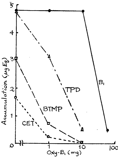
Fig 2 Influence of oxythiamine to the accumulation of thiamine derivatives on Kl. apiculata
