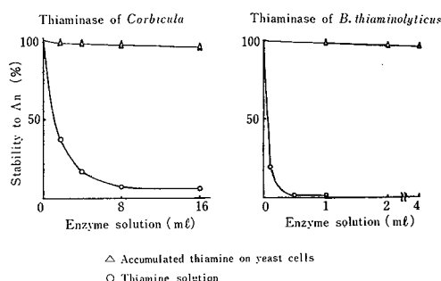
Fig. 1 Stability of accumulated thiamine to thiaminase
