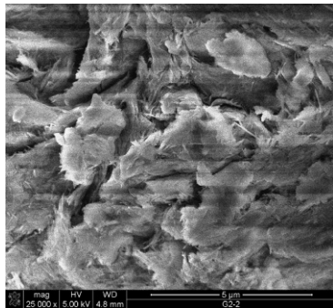
Fig. 3 SEM analyses of Saudi Arabian natural agglomerated nano silicate- aluminum.
