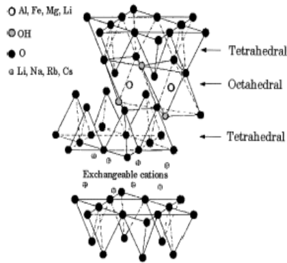
Fig. 1 Silicate-aluminum structure.
