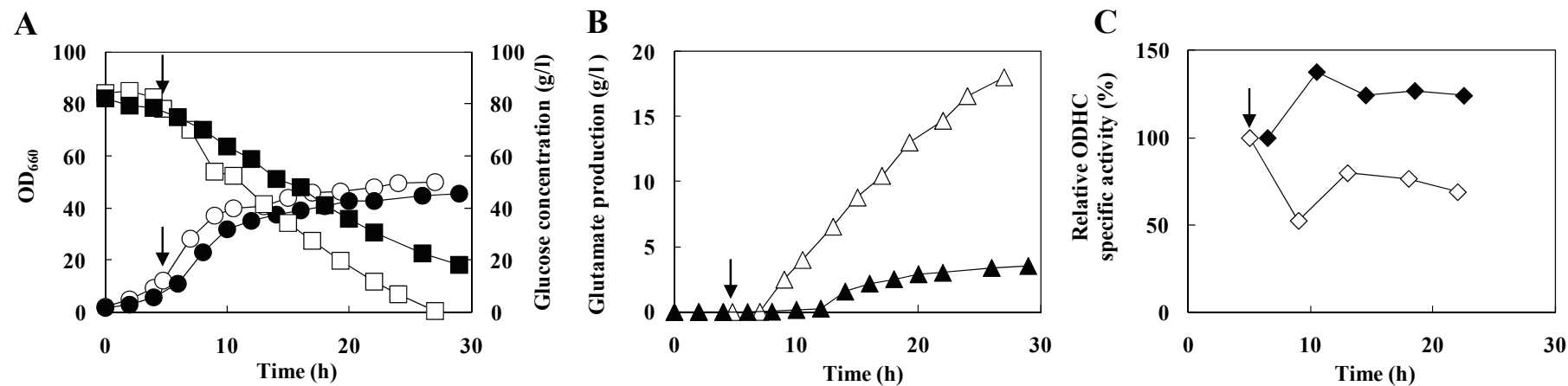
Figure 3.3 Cell growth (A, circles), glucose consumption (A, squares), glutamate production (B, triangles), and relative ODHC specific activity (C, diamonds) of the odhA overexpressing strain ATCC 13032/pECT- odhA (closed symbols) and the control strain ATCC 13032/pECT (open symbols) under Tween 40-triggered glutamate production in jar bioreactor culture. Arrows indicate both IPTG and Tween 40 addition for odhA overexpression and triggering glutamate overproduction, respectively
