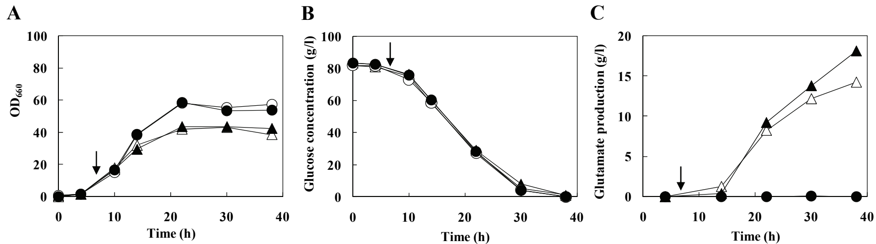
Figure 3.4 Cell growth (A), glucose consumption (B), and glutamate production (C) of the odhA antisense RNA expressing strain ATCC 13032/pECT-Anti- odhA in Sakaguchi flask culture. The representative results of three independent experiments under each culture condition are shown. Arrows Tween 40 and IPTG addition; open circles neither IPTG nor Tween 40 addition; closed circles IPTG addition; open triangles Tween 40 addition; closed triangles both Tween 40 and IPTG addition
