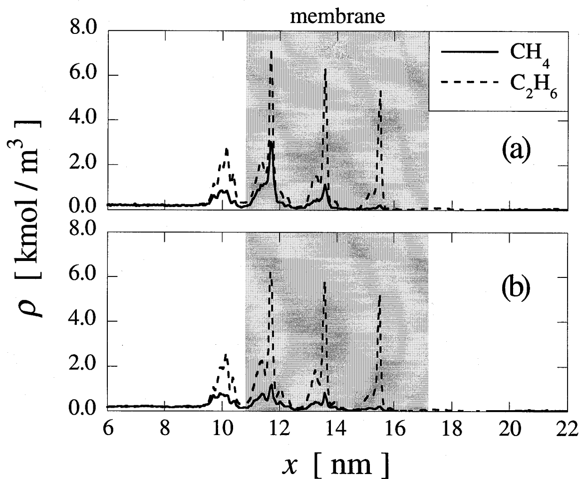
Figure 5-6 Density profiles in the M-region for (a) pure and (b) mixed-gas permeation through pore B of the diamond path membrane; solid lines denote \text{CH}_4 and broken lines \text{C}_2\text{H}_6 ; \Delta P = 0.5 MPa for pure gases, \Delta P_k = 0.5 MPa for mixed gas, T = 300 K
