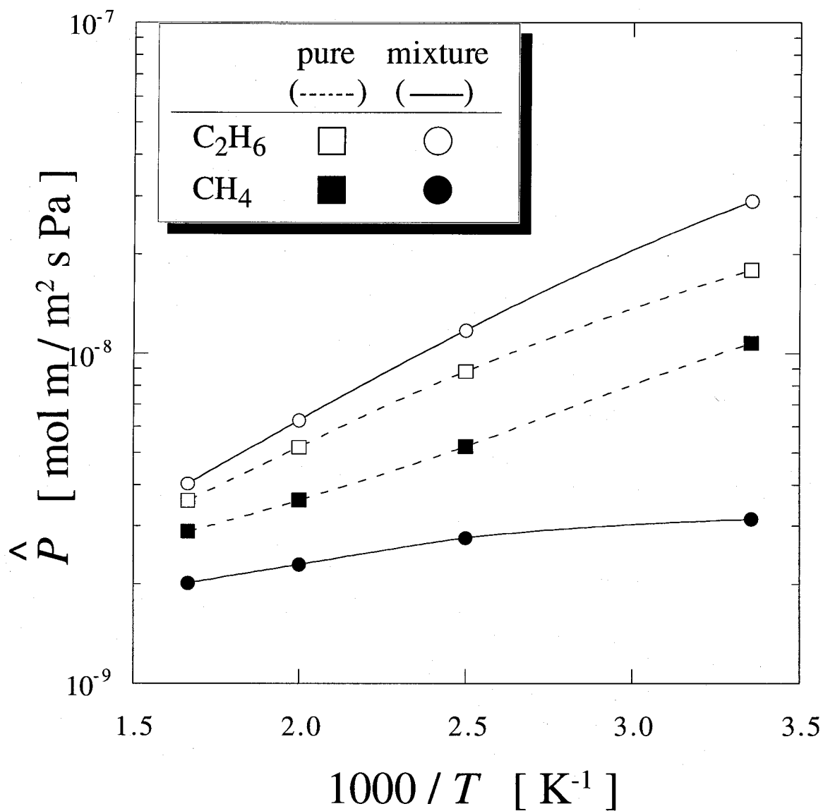
Figure 2-8. Temperature dependance of permeability of CH 4 and C 2 H 6 for pure and equimolar mixed gases at \Delta P = 0.5 MPa for a slit pore of W_p^* = 6
