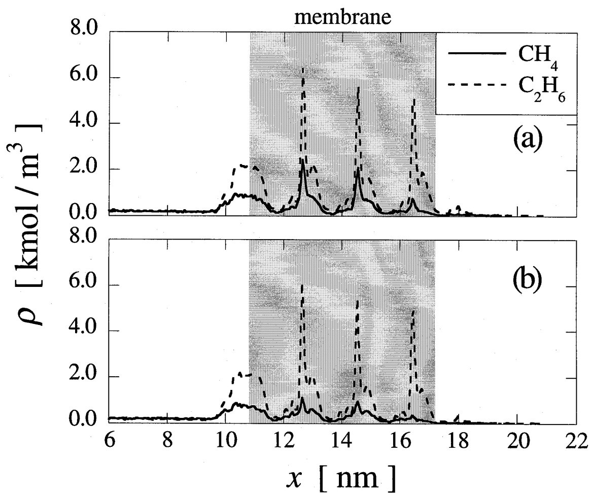
Figure 5-5 Density profiles in the M-region for (a) pure and (b) mixed-gas permeation through pore A of the diamond path membrane; solid lines denote \text{CH}_4 and broken lines \text{C}_2\text{H}_6 ; \Delta P = 0.5 MPa for pure gases, \Delta P_k = 0.5 MPa for mixed gas, T = 300 K
