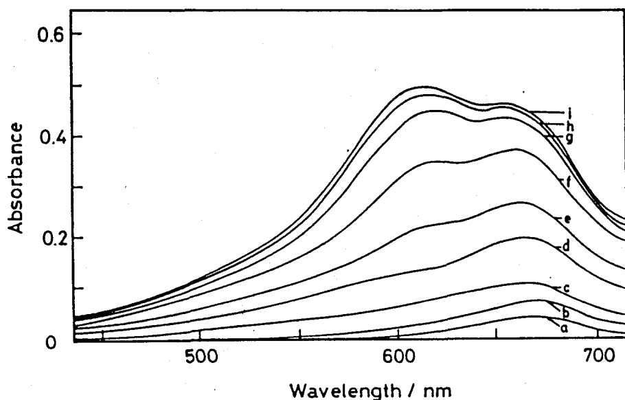
Fig. 40. Absorption spectra of MB-incorporated Naflon/ITO electrode polarized at 0.10 (a), 0.26 (b), 0.28 (c), 0.30 (d), 0.32 (e), 0.34 (f), 0.36 (g), 0.38 (h), and 0.5 (i) V vs. SCE in 0.5 M \text{H}_2\text{SO}_4 . The MB incorporation was performed by immersing Naflon/ITO in 1.0 \times 10^{-3} M MB solution for 30 min.
