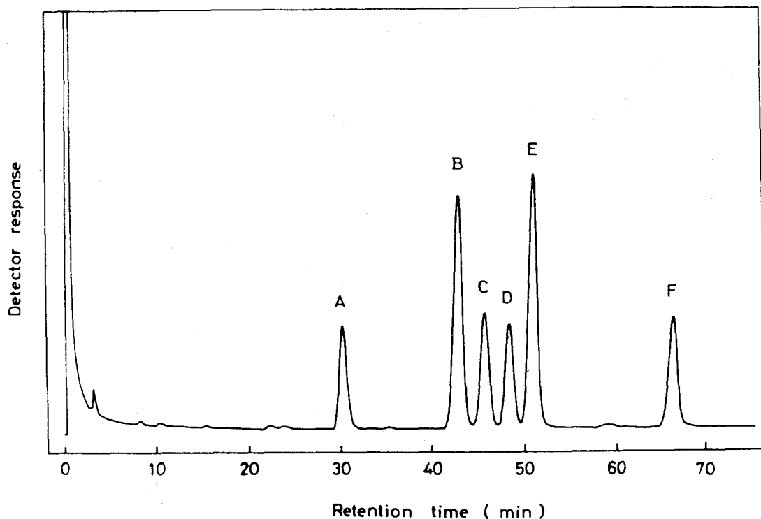
Fig. 4-1. Gas-liquid chromatogram of the alditol acetates of methylated sugars from depyruvylated succinoglycan on an OV275-GEXF1150 column.
