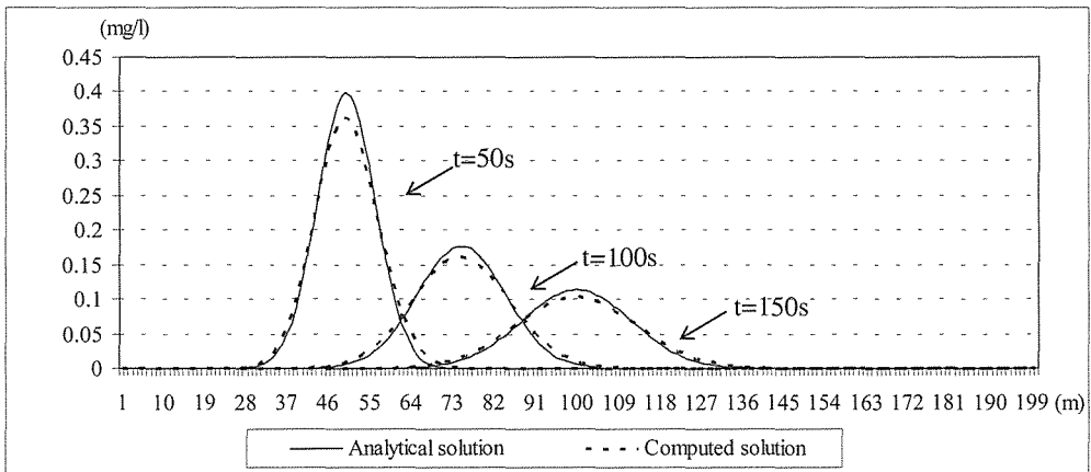
Fig. 2. Concentration distribution along a ray passing the source point and parallel with the flow direction, at t = 50 \text{ s} , t = 100 \text{ s} and t = 150 \text{ s} .
