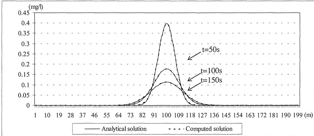
Fig. 1. Concentration distribution along a ray passing the source point and parallel with the Ox axis, at t = 50 \text{ s} , t = 100 \text{ s} and t = 150 \text{ s}
