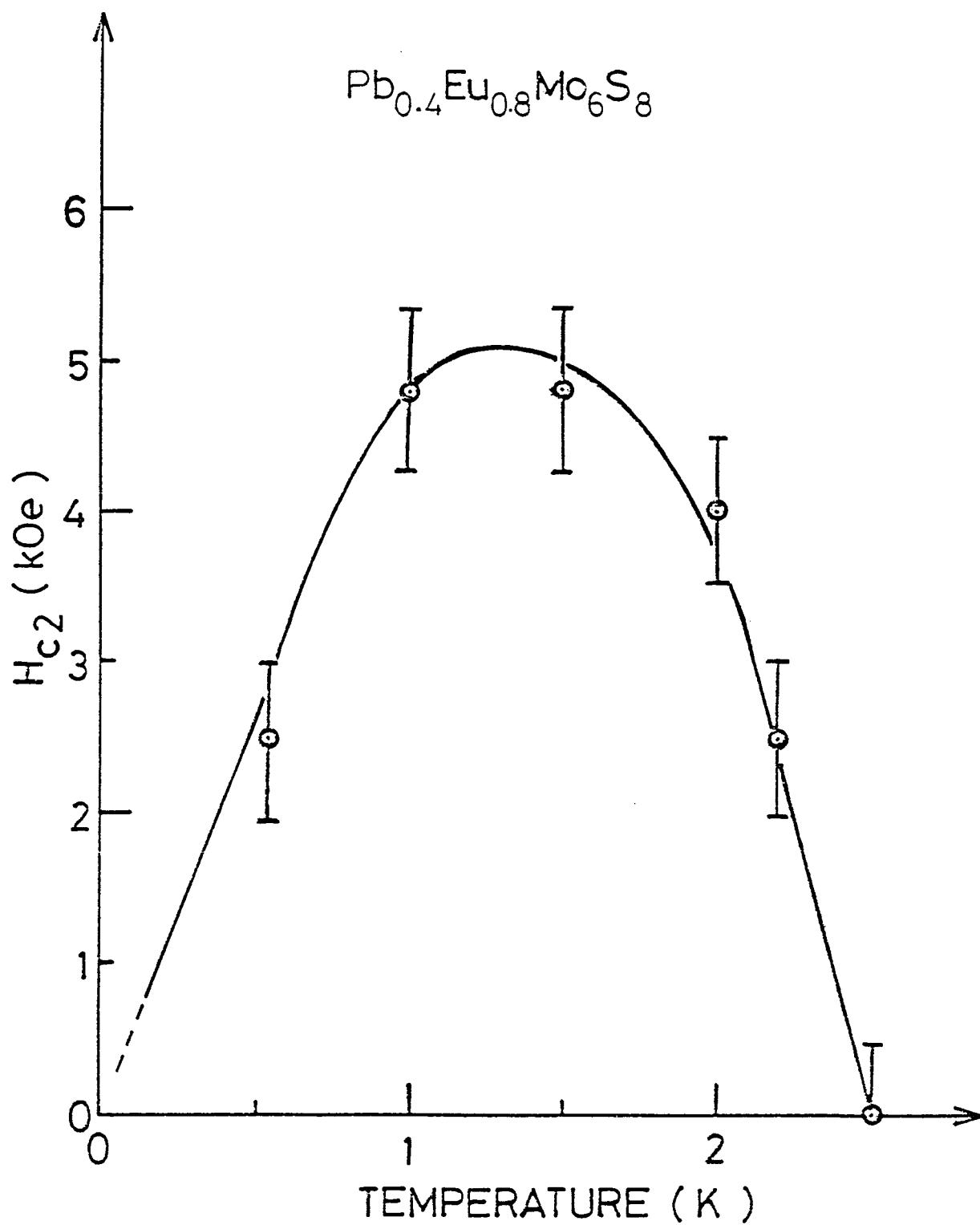
FIG.29 Temperature dependence of H_{c2} in \text{Pb}_{0.4}\text{Eu}_{0.8}\text{Mo}_6\text{S}_8 .
