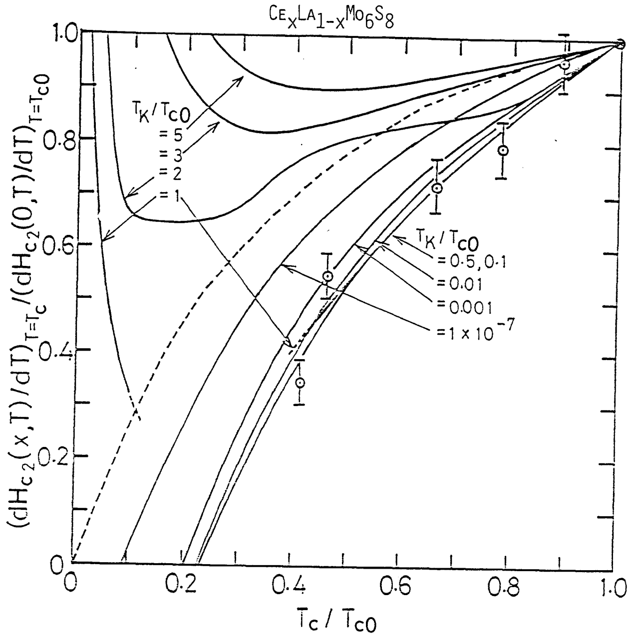
FIG.12 The initial slope of the H_{c2}(T) curve, (dH_{c2}/dT)_{T_c} as a function of reduced temperatures T_c/T_{c0} . The initial slope is also reduced by that of \text{LaMo}_6\text{S}_8 . Solid lines are calculated by the theory of MIN. 16) A broken line is for the AG theory 6) . The MIN curves obtained by numerical calculations are unstable in the low-temperature region for T_K/T_{c0} \sim 1 , so they are not shown in the figure.
