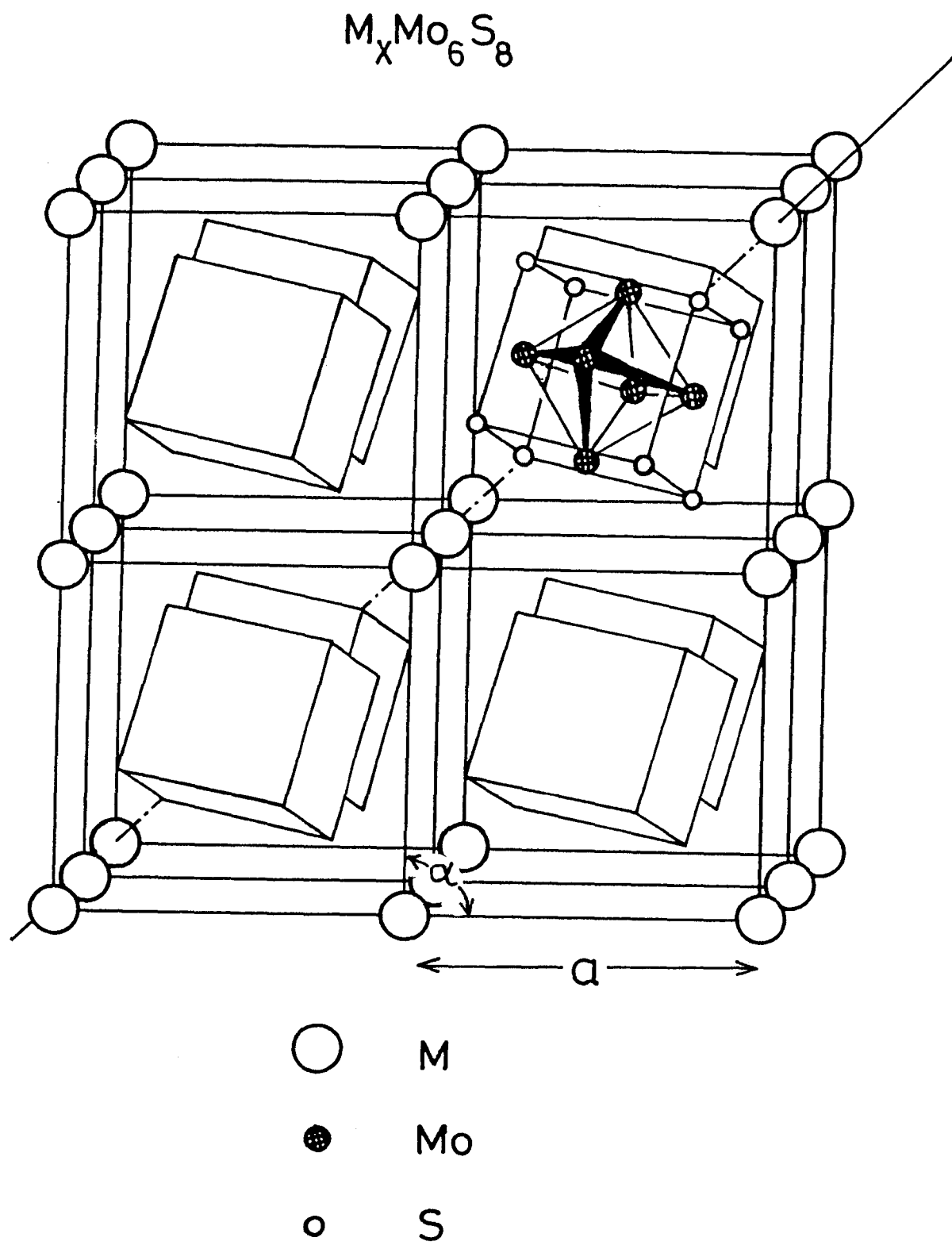
Fig.4 Crystal structure of M_x Mo_6 S_8
