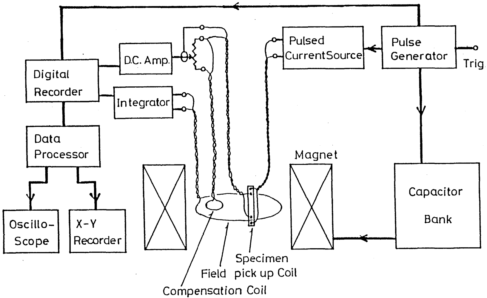
Fig.11 Block diagram of magnetoresistance measurement under a pulsed magnetic field.
