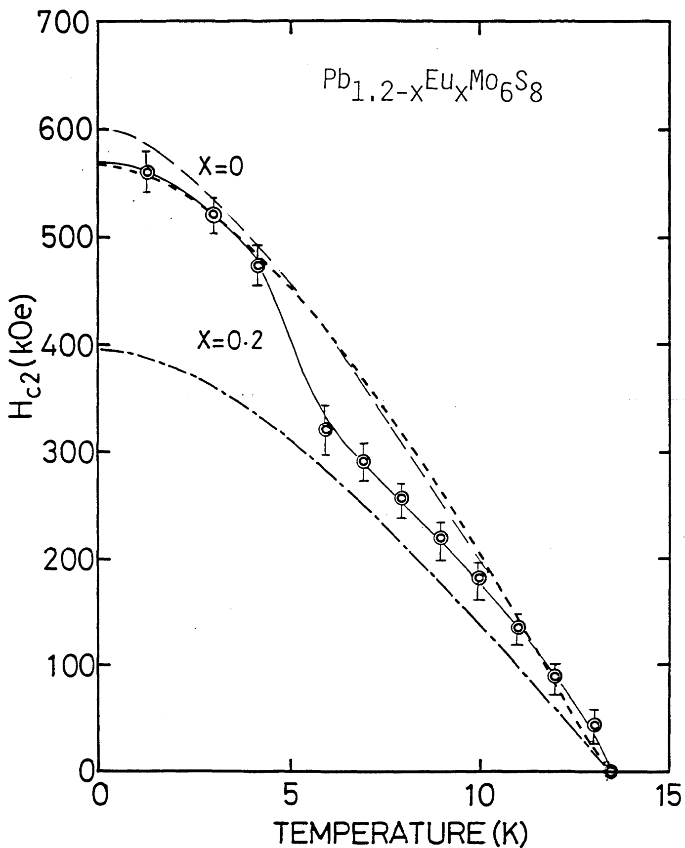
FIG.27(a) Temperature dependence of H_{c2} in \text{Pb}_{1.2-x}\text{Eu}_x\text{Mo}_6\text{S}_8 for x = 0.2 . A dashed line is for x = 0 . Broken line and dash-dotted line are the theoretical curves as given in the text.
