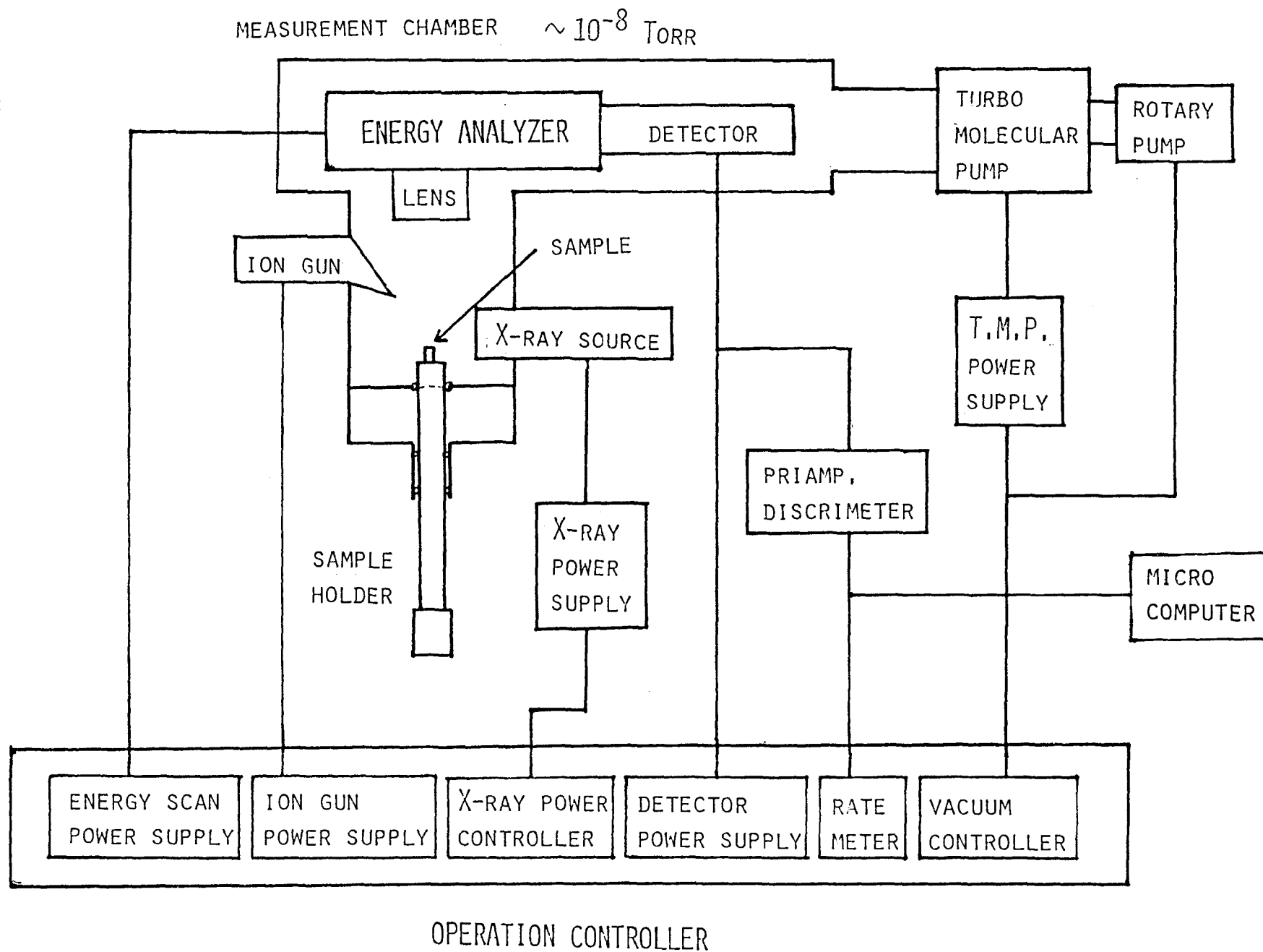
Fig.5 Block diagram of XPS measurement ( ESCA 750 )
