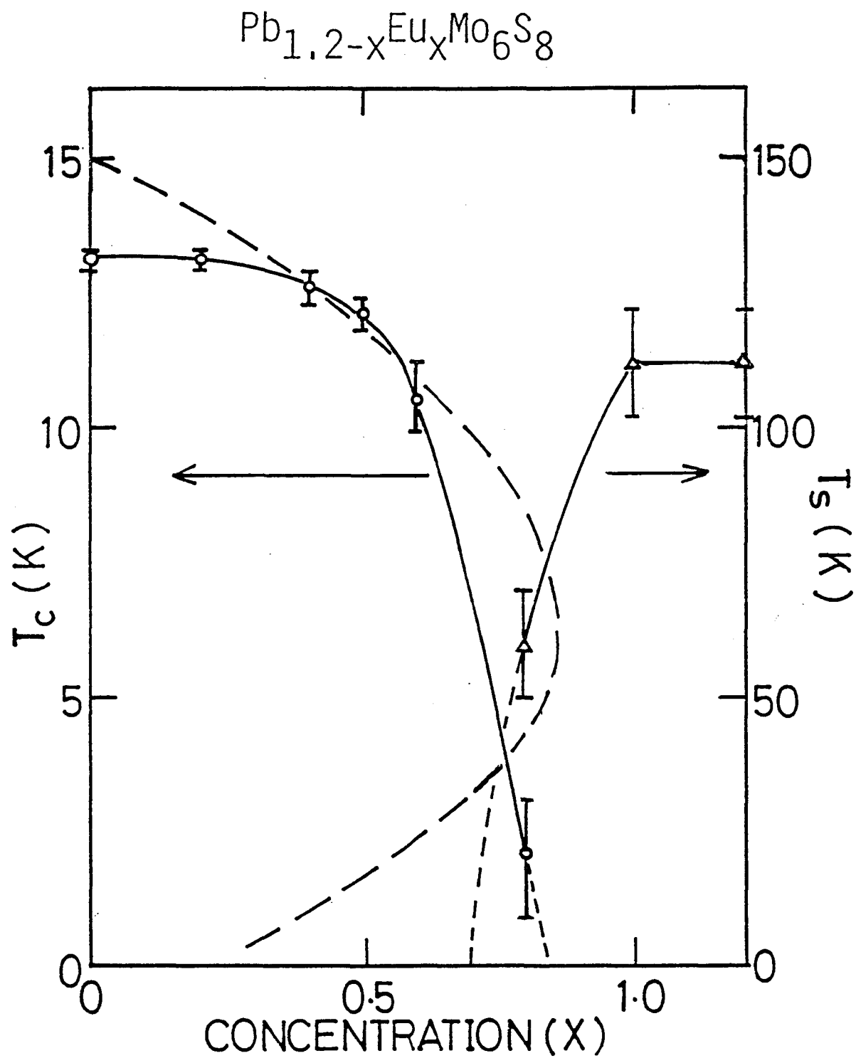
FIG.22 Eu concentration dependence of superconducting transition temperature T_c and structural transformation temperature T_s . A broken line is the theoretical curve of T_c(x) .
