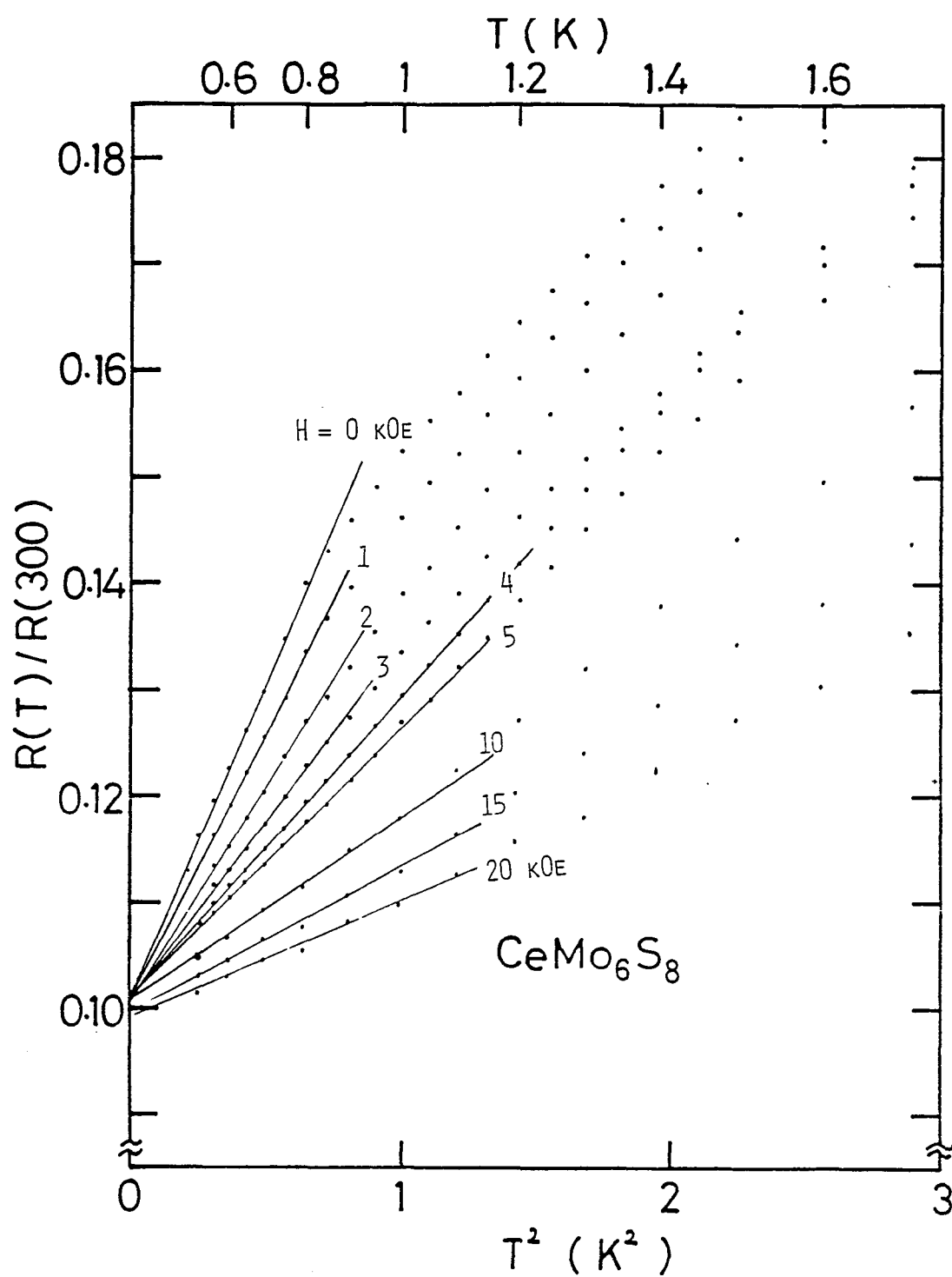
FIG.23 Magnetoresistance of CeMo_6S_8 as a function of T^2
