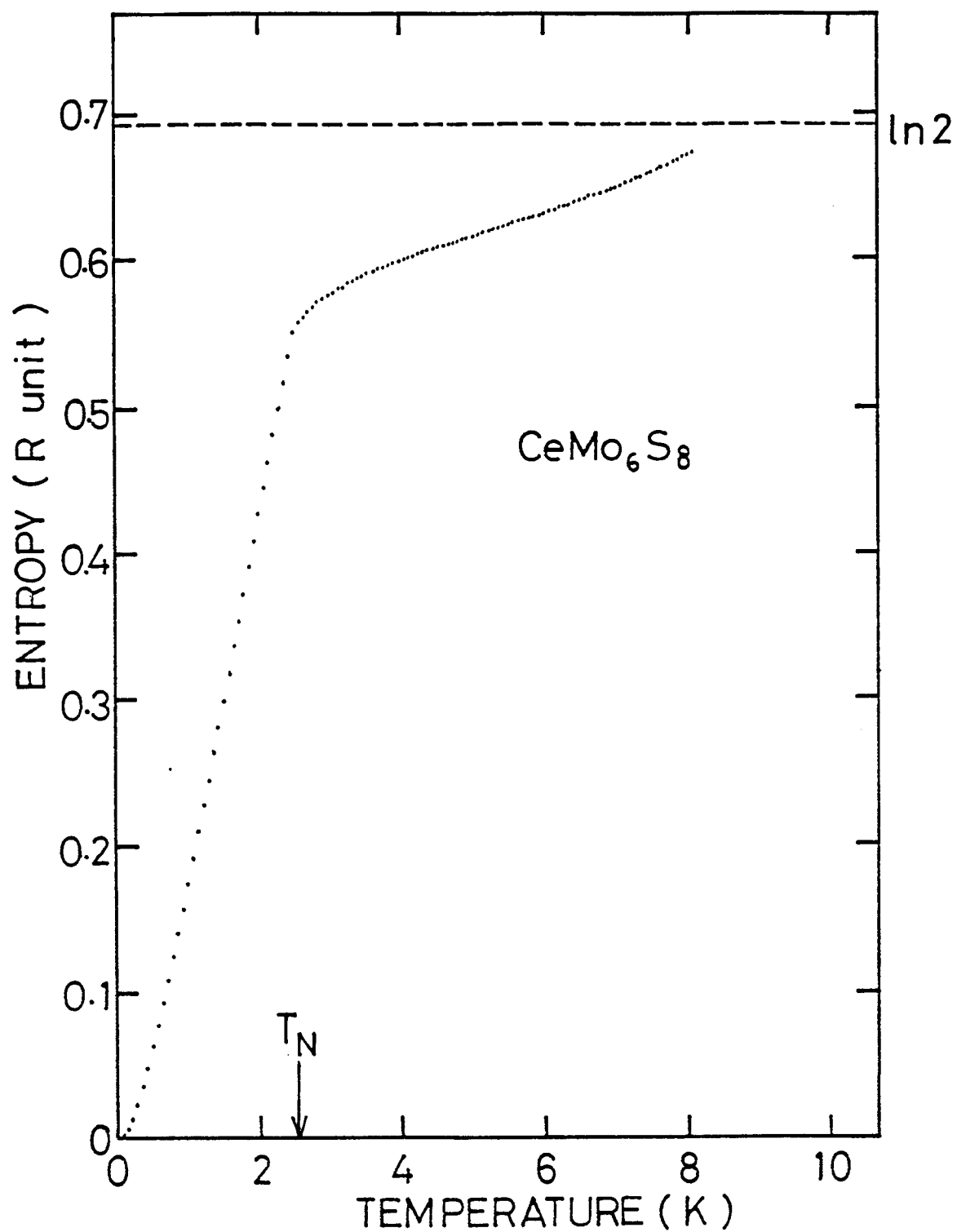
FIG.18 Temperature dependence of magnetic entropy of \text{CeMo}_6\text{S}_8 from the data of magnetic specific heat measurement by Maple et al. 3) ( see Fig.1 ).
