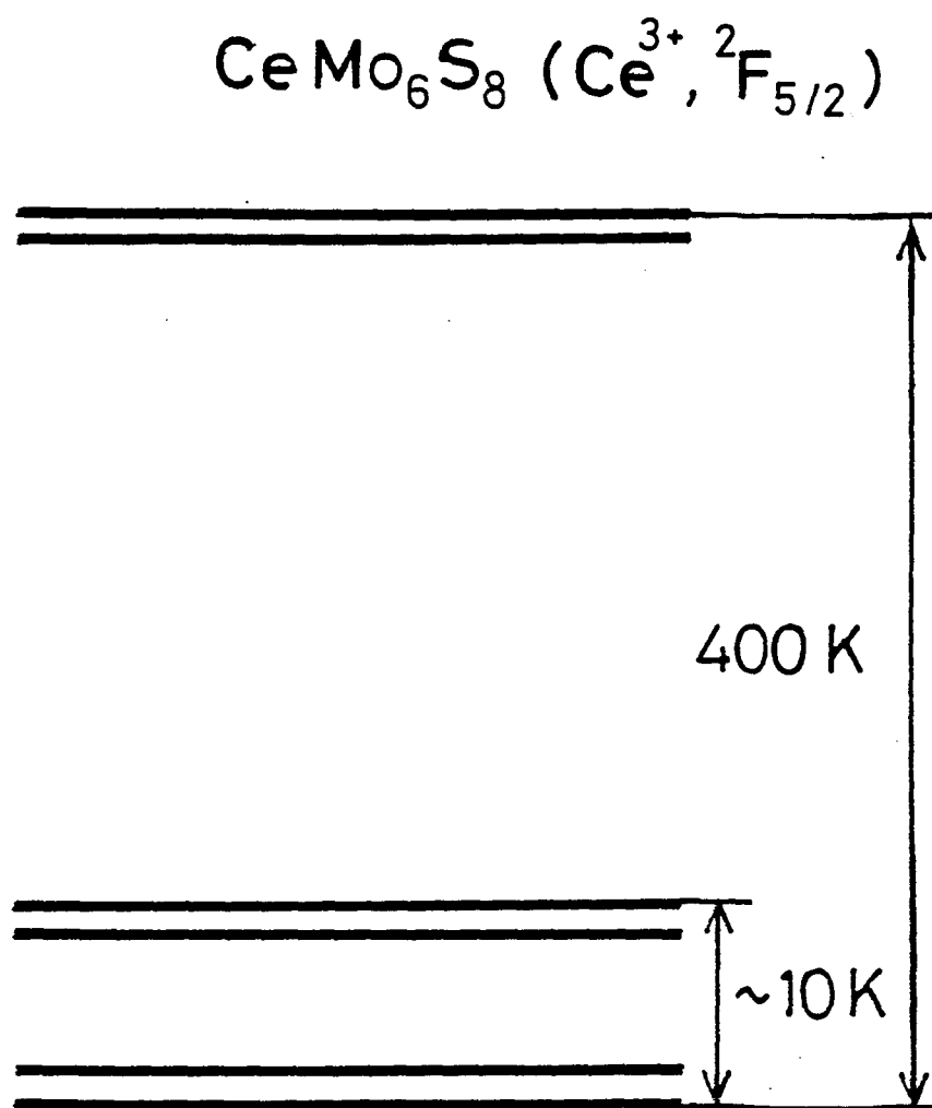
FIG.19 Crystal field splitting of \text{CeMo}_6\text{S}_8 proposed in the present work.
