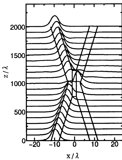
(c) P_1 = 20.8\text{mW/mm}
