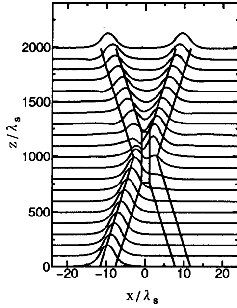
(b) P_{3c} = 11.8 \text{ mW/mm}
