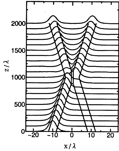
(b) P_1 = 28.6\text{mW/mm}
