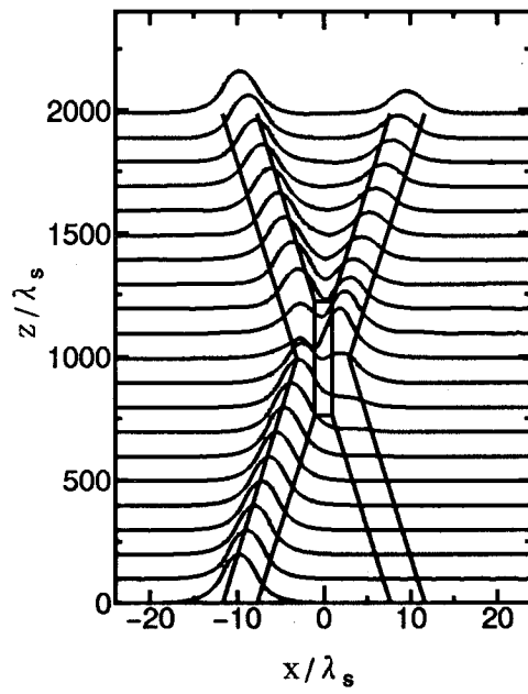
(c) P_{3c} = 15.6 \text{ mW/mm}
