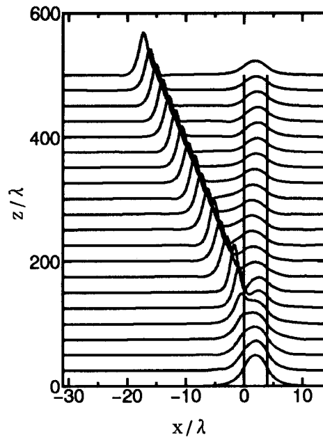
(a) \Delta z = 0.01\lambda
