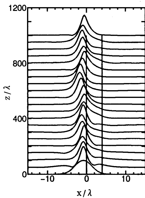
(c) 2w_0 = 6\lambda
