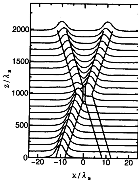
(b) P_{3c} = 20.8 \text{ mW/mm}
