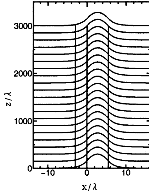
(a) P_{in} = 2.0 \text{ mW/mm}
