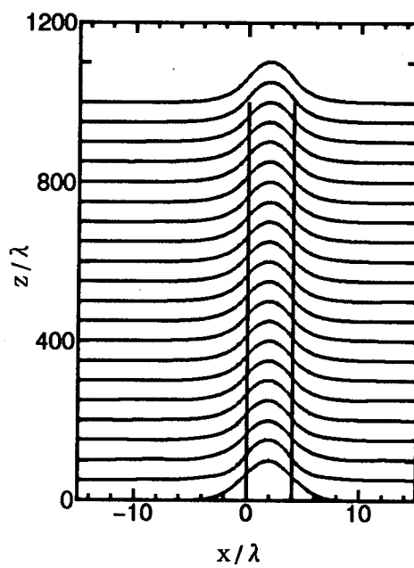
(b) 2w_0 = 6\lambda
