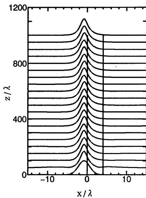
(b) 2w_0 = 4\lambda
