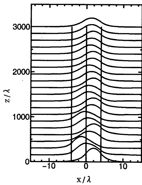
(b) P_{in} = 40.0\text{mW/mm}
