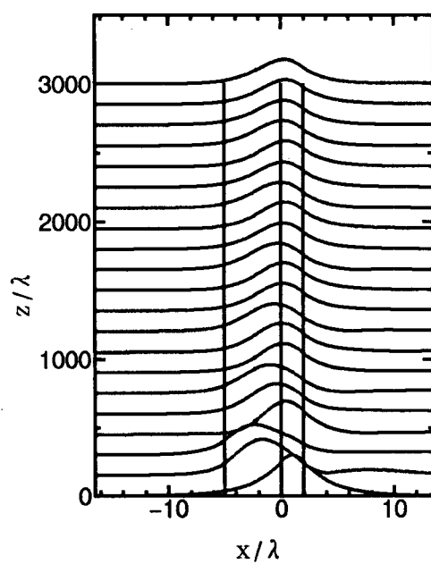
(b) P_{in} = 30.0 \text{ mW/mm}
