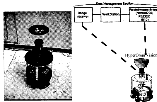
Fig.6 System Configuration
