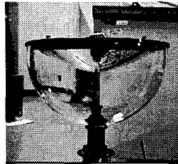
Fig. 1 HyperOmniVision
