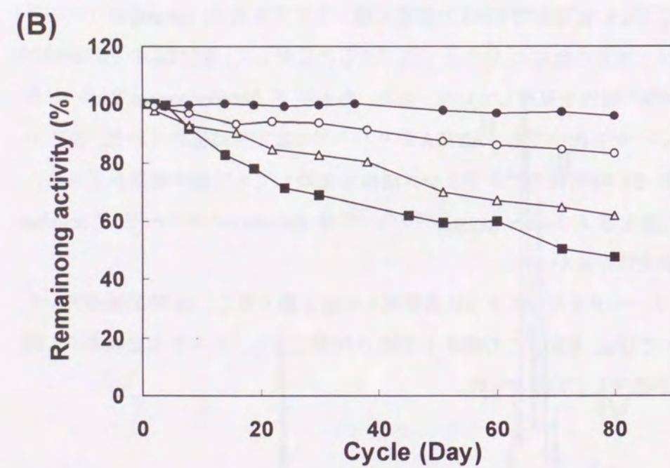
Fig. 6-4. Stability of various immobilized lipases in acidolysis of tripalmitin with oleic acid. The acidolysis was conducted under the conditions described in Fig. 6-2, and repeated by transferring the immobilized lipase to a fresh substrate mixture every 24 h. (A) Activity of immobilized lipase after 3-h reaction; (B) after 24-h reaction. ●, F. heterosporum R275A lipase; ○, F. heterosporum wild lipase; △, R. delemar lipase; ■, Lipozyme IM60.
