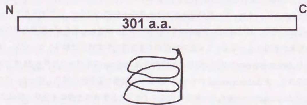
Fig. 4-6. Schematic structure of lipases A and B. The arrow indicate the cleavage site by a trypsin-like protease. N, N-terminus; C, C-terminus; a.a., amino acid residues.
