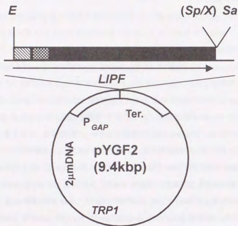
Fig. 3-1. Structure of plasmid pYGF2. Restriction sites are abbreviated as follows; E, EcoRI ; Sp, SpeI ; Sa, SaI ; X, XbaI . The promoter and terminator are shown as P_{GAP} and Ter., respectively. The hatched box, dotted box, and solid box are signal, pro, and mature sequence of F. heterosporum lipase, respectively. The transcriptional direction is indicated by an arrow. The 2 \mu mDNA replication origin and complementary gene of trp1 in the host strain are shown as 2 \mu mDNA and TRP1 , respectively.
