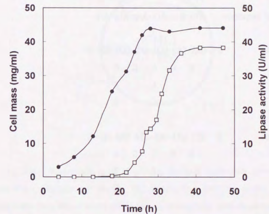
Fig. 2-1. Time course of lipase production by F. heterosporum . Cultivation was carried out at 25°C in 500 ml flask with 70 ml of 3%soybean oil, 4%corn steep liquor, 0.1%yeast extract, 0.1%KH 2 PO 4 , 0.05%MgSO 4 ·7H 2 O (pH 5.5). ●; Cell mass (wet wt.), □; lipase activity in the culture broth.
