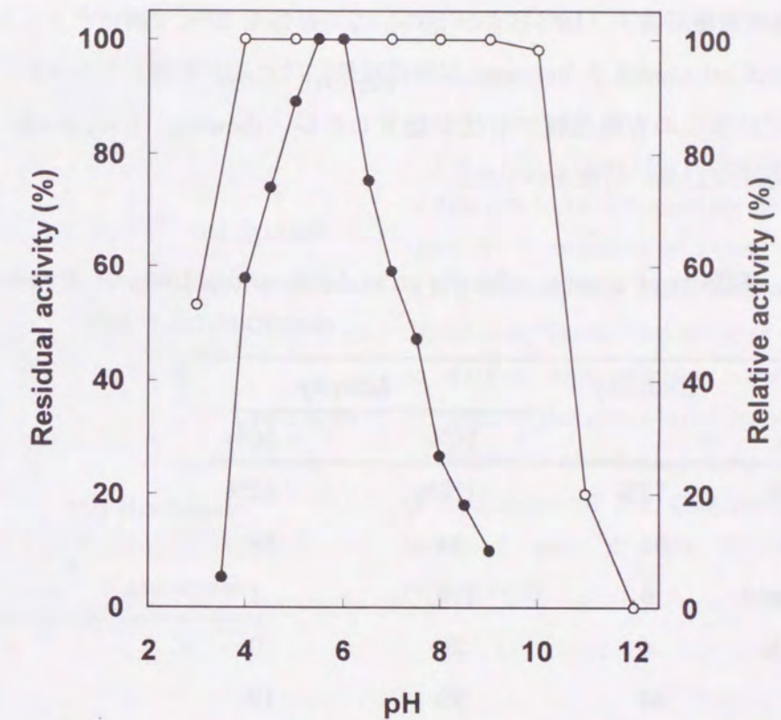
Fig. 1-5. pH stability (○) and optimum pH (●) of F. heterosporum lipase. The remaining activity was measured after incubation in Briton-Robinson buffer at 40°C for 4h. Briton-Robinson buffer was used for the optimum pH at 30°C.
