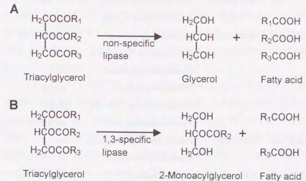
Fig.1. Reaction of lipase.
