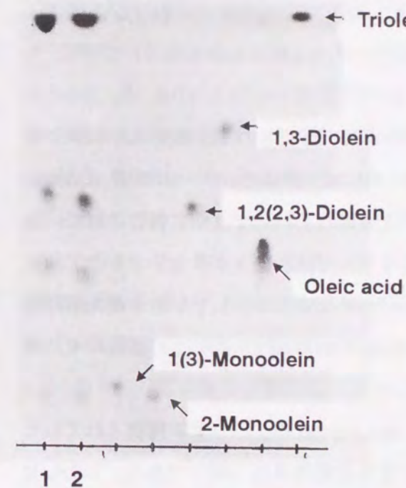
Fig. 1-6. Thin-layer chromatography of the products obtained by hydrolysis of triolein. A reaction mixture containing 0.1 g triolein was incubated at 40°C for 10-20 min. Then, 7 ml of ether was added to extract the reaction products, and aliquots of the ether layer were subjected to thin-layer chromatography. The extent of hydrolysis of the samples applied to lanes 1 and 2 was 10 and 14%, respectively.
