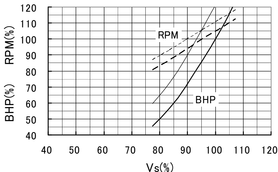
Fig. 3.3 BHP increase and RPM increase at the same V_s
