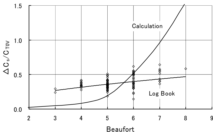
Fig. 6.9 Comparison of \Delta C_s/C_{to} between log book analysis data by eq(6.6) and calculation result, ship A
