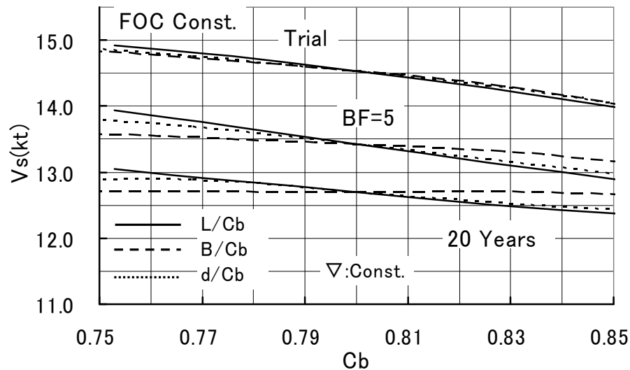
Fig. 7.5 Ship speed in ship S' group of the same \nabla at constant FOC
