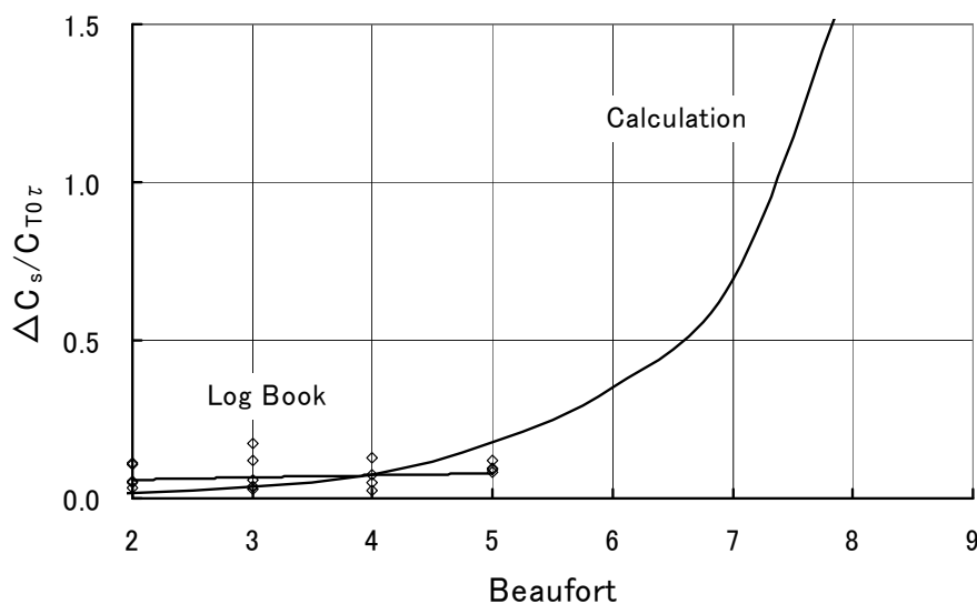
Fig. 6.10 Comparison of \Delta C_s/C_{to} between log book analysis data by \tau and calculation result, ship B
