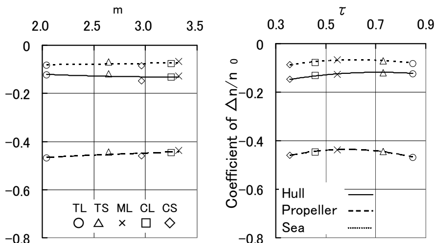
Fig. 4.15 Relation between the coefficient of \Delta n/n_0 and m , \tau
