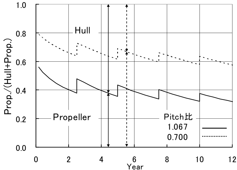
Fig. 4.17 Ratio of hull and propeller in speed drop
