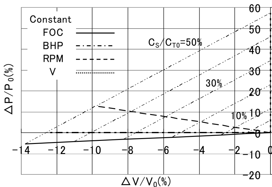
Fig. 4.19 \Delta P/P_0 versus \Delta V/V_0 in different engine condition
