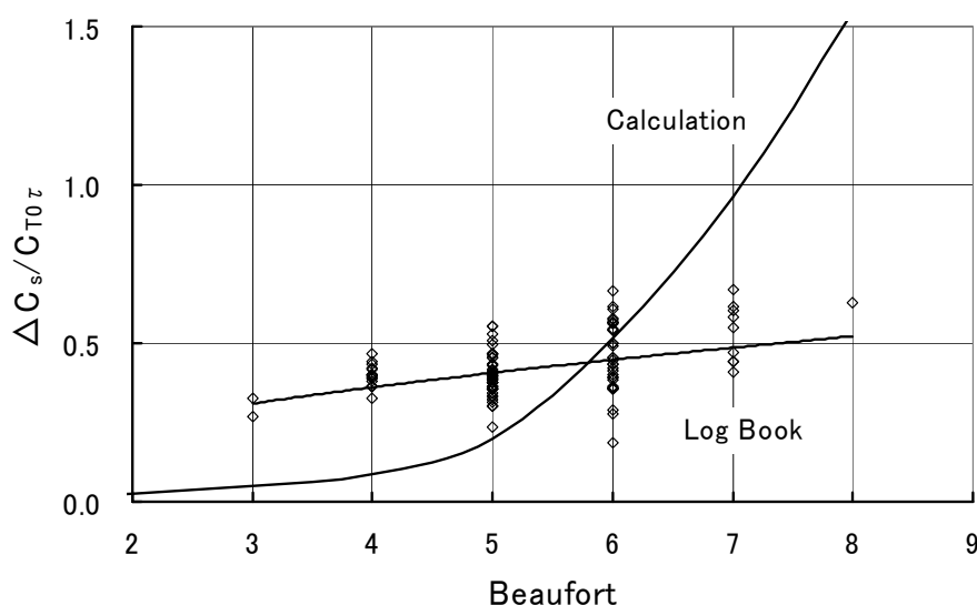
Fig. 6.8 Comparison of \Delta C_s/C_{T0} between log book analysis data by \tau and calculation result, ship A
