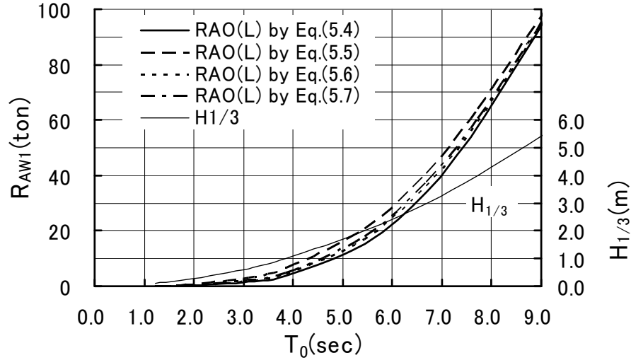
Fig. 5.2 Comparison of R_{AW1}(\text{ton}) with different \alpha_2
