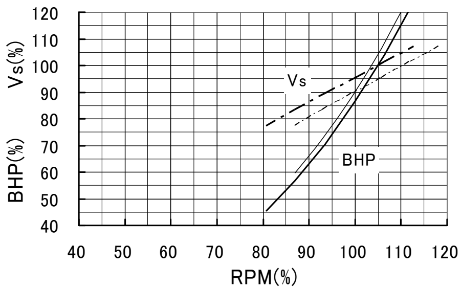
Fig. 3.4 BHP increase and Vs decrease at the same RPM
