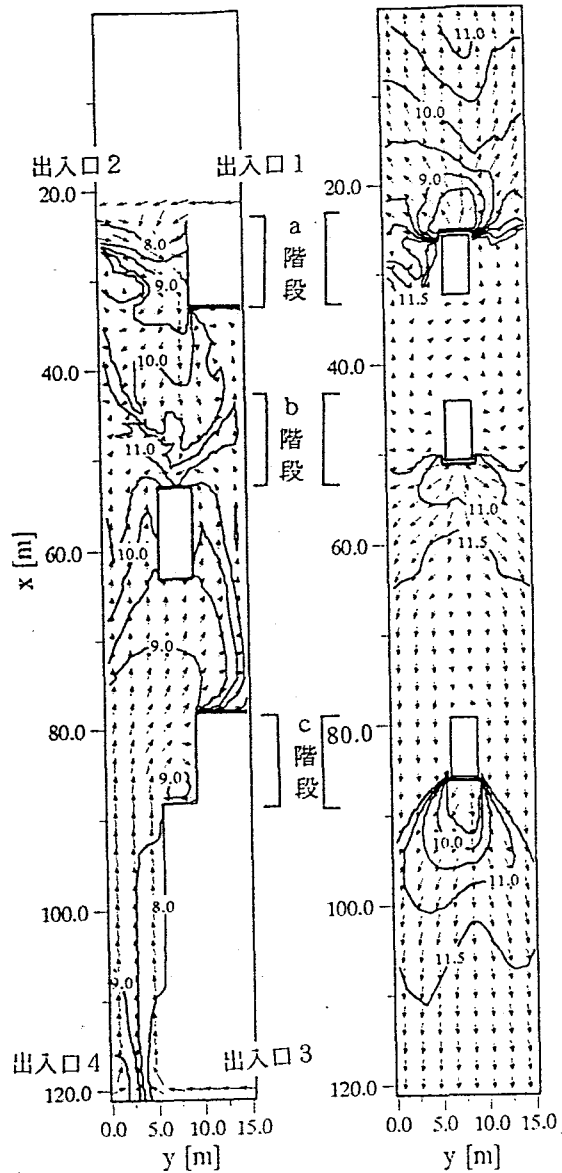
図-4.20 気流・気温分布図 (t=50s)
