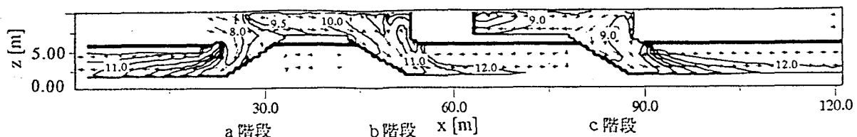
図-4.20 気流・気温分布図 (t=50s)
