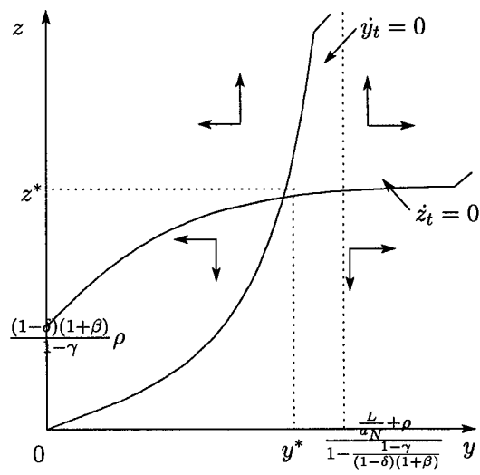
Fig. 1. The phase diagram
