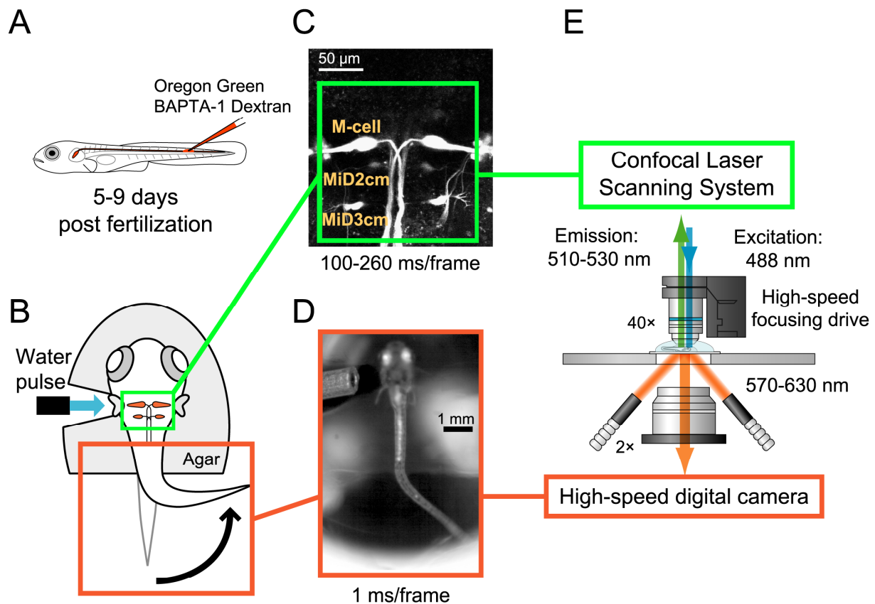
Figure. 1-1. Experimental setup for simultaneous monitoring of RS neuron activity and behavior. A , RS neurons were labeled retrogradely with a fluorescent Ca 2+ indicator, Oregon Green BAPTA-1 dextran, injected into caudal spinal cord. B-E , The rostral body, anterior to the cloaca, of the larval zebrafish was embedded in agar ( B ). A water pulse was usually applied to the otic vesicle (OV; a premature organ of inner ear). The evoked fluorescence responses in the RS neurons (green) and tail movement (orange) were monitored simultaneously with confocal microscopy ( C and E , upright optics) and a high-speed digital camera ( D and E , inverted optics), respectively. The tail of the semi-fixed larva was illuminated with orange light that did not interfere with confocal imaging. The high-speed focusing drive, which enabled us to switch focal planes alternately during image acquisition, was used in Chapter 2 and 3. See Materials and Methods for detail.
