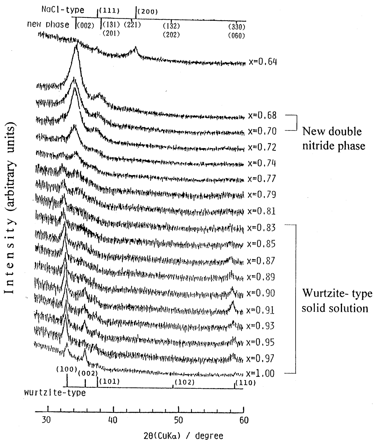
Fig.3-2-1. X-ray diffraction patterns of \text{Ti}_{1-x}\text{Al}_x\text{N} films in the 0.64 \leq x \leq 1.00 range
