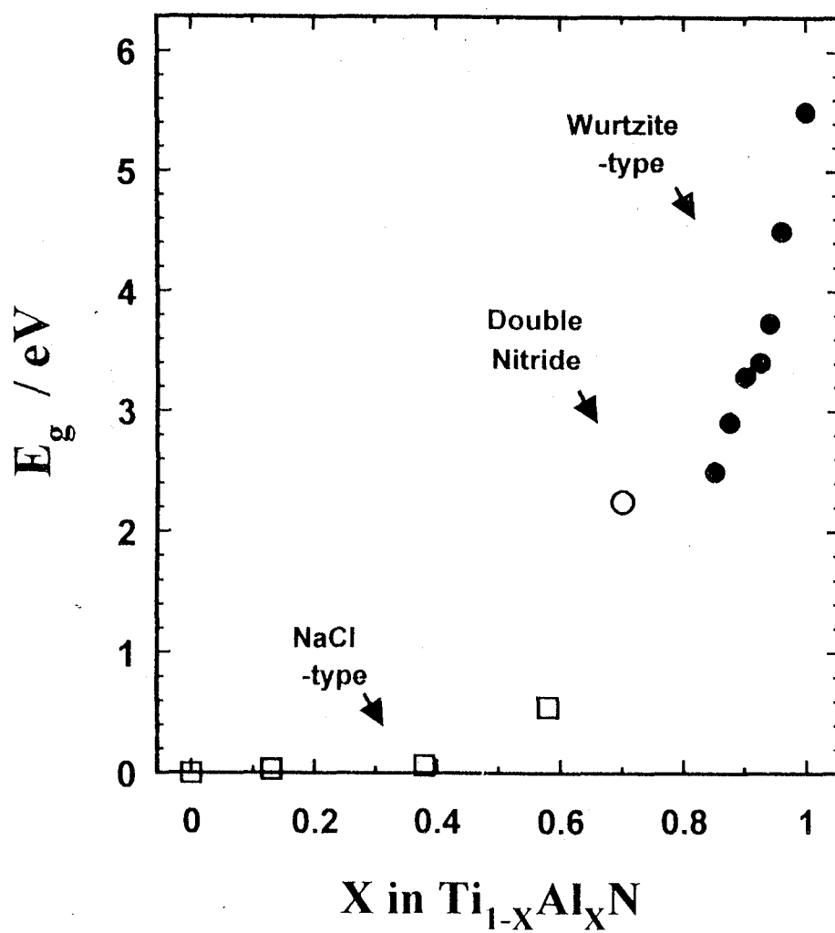
Fig.4-5-1. Band gap of \text{Ti}_{1-x}\text{Al}_x\text{N}
