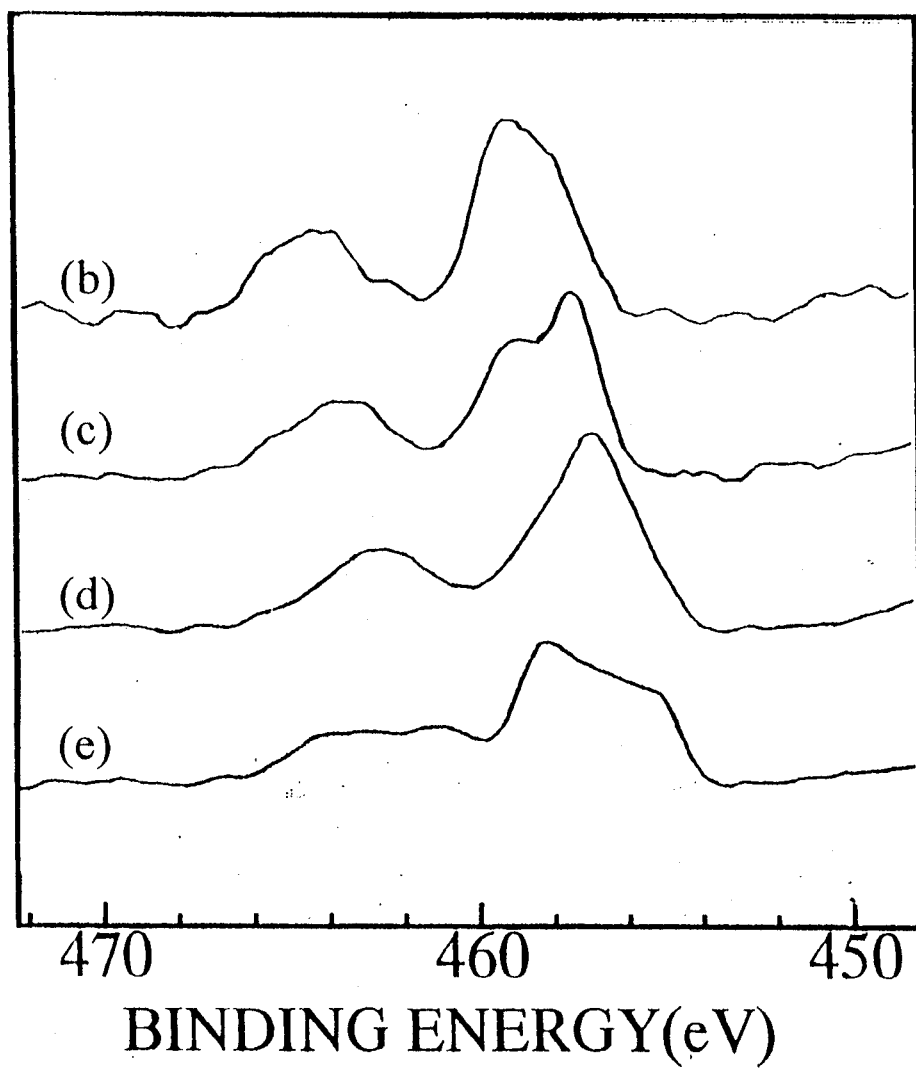
Fig.3-5-1. Ti 2p, XPS of \text{Ti}_{1-x}\text{Al}_x\text{N} surface
