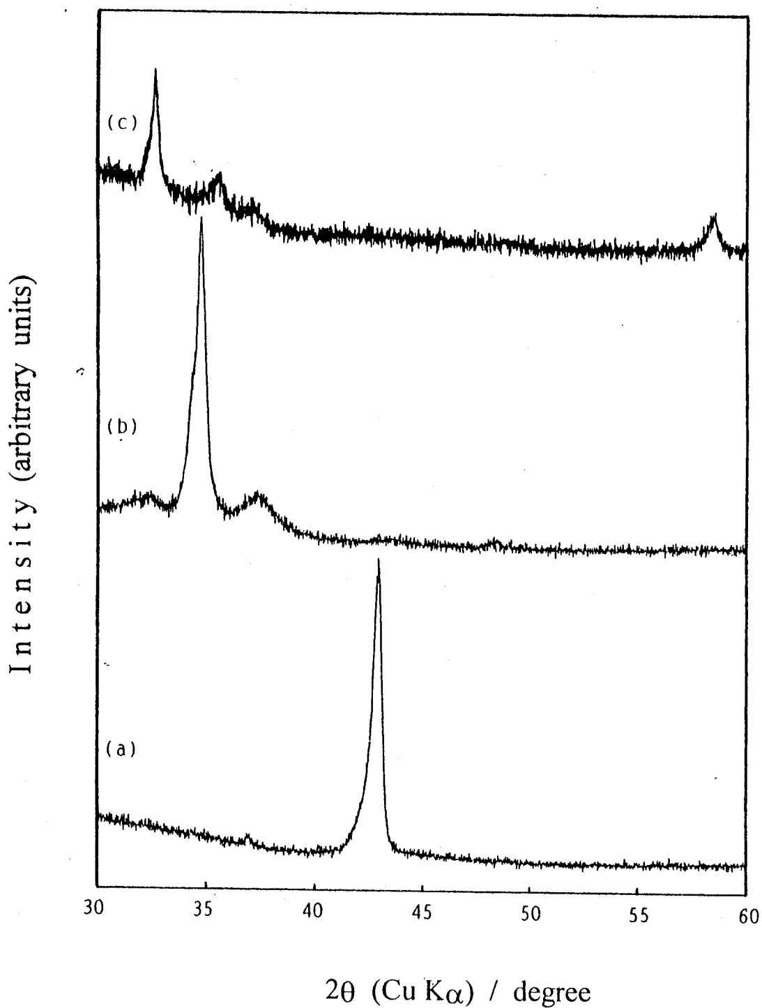
Fig.2-4. X-ray diffraction patterns of \text{Ti}_{1-x}\text{Al}_x\text{N} solid solutions: a) NaCl- type solid solution ( x = 0.5 ) b) New double nitride ( x = 0.7 ) c) Wurtzite- type solid solution ( x = 0.85 )
