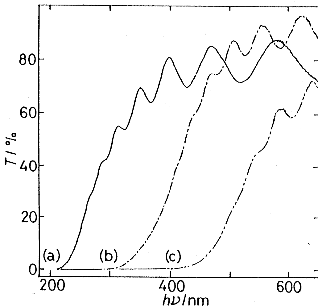
Fig. 4·2·1. UV Spectra for some of \text{Ti}_{1-x}\text{Al}_x\text{N} solid solutions. (a) x=1.0 , (b) x=0.90 , and (c) x=0.83 . The ordinate denotes transmittance, T .
