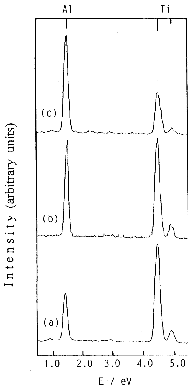
Fig.2-5. Analytical electron microscope traces of \text{Ti}_{1-x}\text{Al}_x\text{N} solid solutions:
