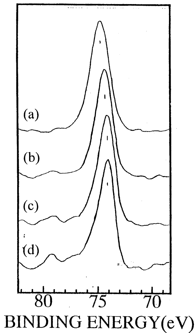
Fig.3-5-3. Al 2p, XPS of Ti_{1-x}Al_xN after 15 min. etching
