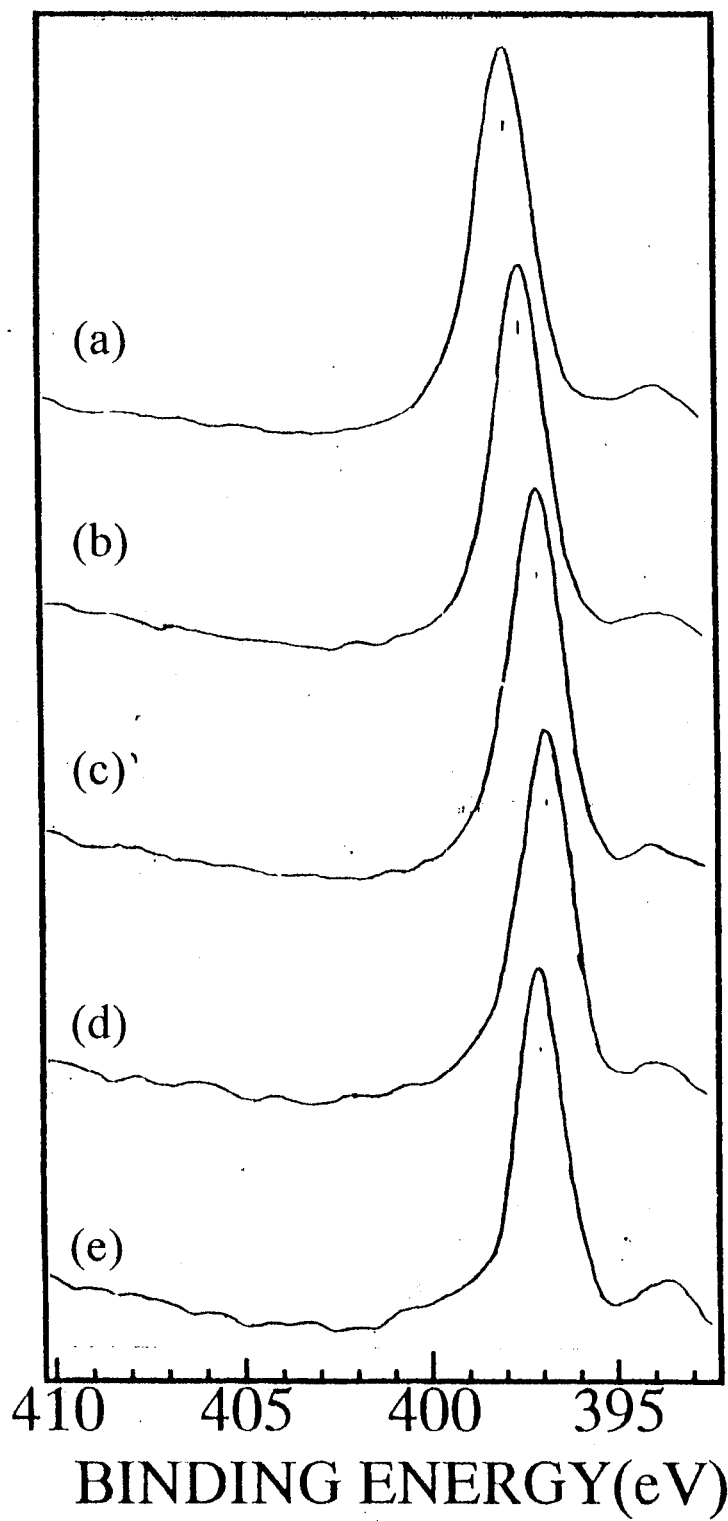
Fig.3-5-4. N 1s, XPS of \text{Ti}_{1-x}\text{Al}_x\text{N} after 15 min. etching
