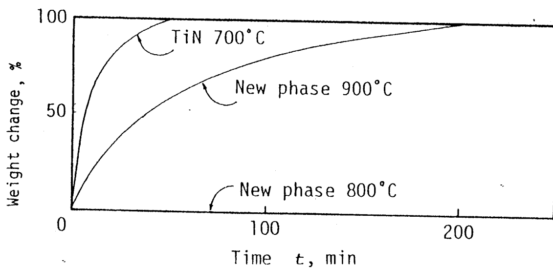
Fig. 4.3.4. Weight change of TiN and new phase with heating time at constant temperature in O_2 gas flow.
