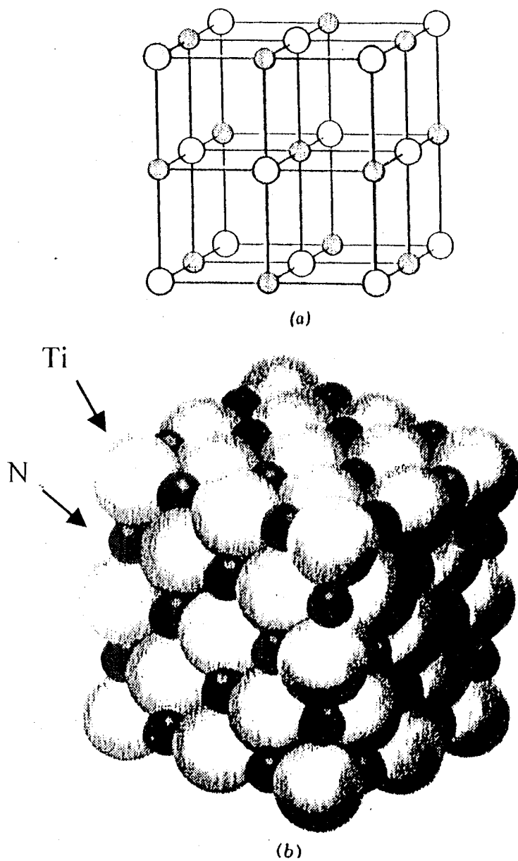
Fig.1-2. Crystal structure of TiN (sodium chloride like structure) \text{Ti} \rightarrow \text{Cl}^- , \text{N} \rightarrow \text{Na}^+
