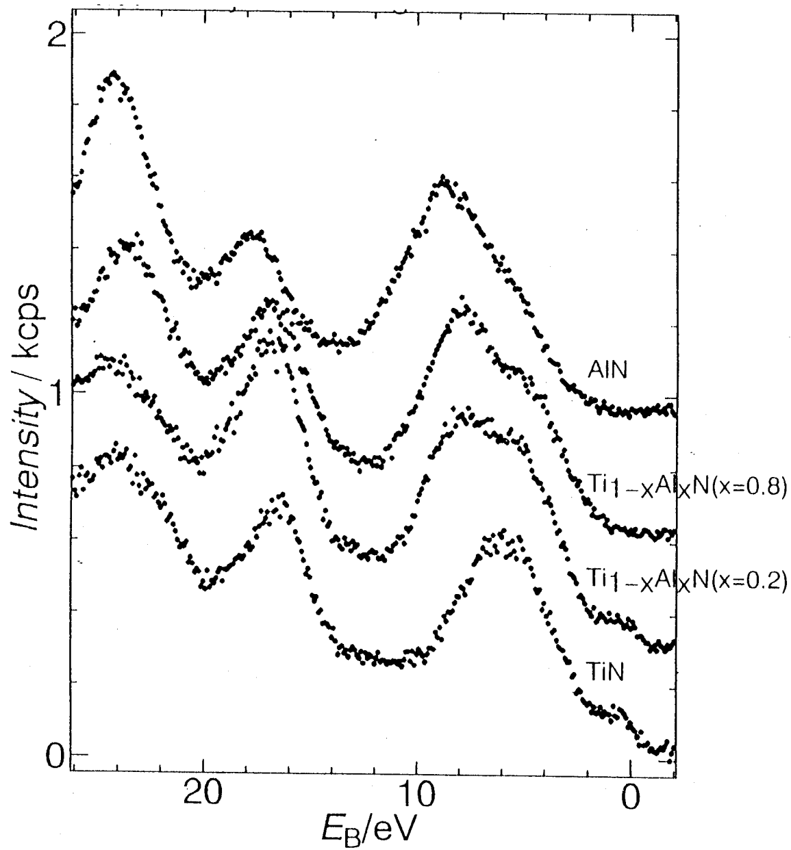
Fig.3-5-5. VB region of XPS for Ti_{1-x}Al_xN thin film cleanned up by means of Kr^+ etching
