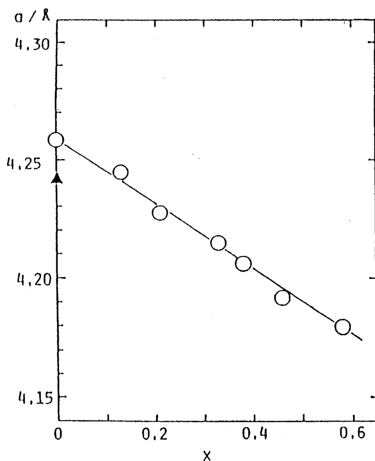
Fig. 3-1-4. Relationship between lattice constant and composition of \text{Ti}_{1-x}\text{Al}_x\text{N} with NaCl-type structure. ○: sputtered films at gas pressure 1 \times 10^{-2} Torr, ▲: reported value at ASTM card 6-0644.
