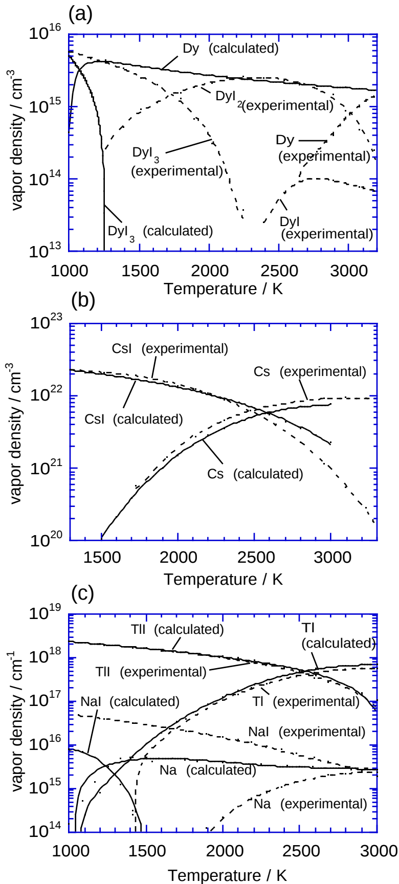
Figure 4.2 Vapor densities of the metal and iodides in (a) \text{DyI}_3/\text{Hg} , (b) \text{CsI}/\text{Hg} , and (c) \text{TlI}/\text{NaI}/\text{Hg} arc discharge lamps as a function of temperature. The solid and dashed lines denote the
