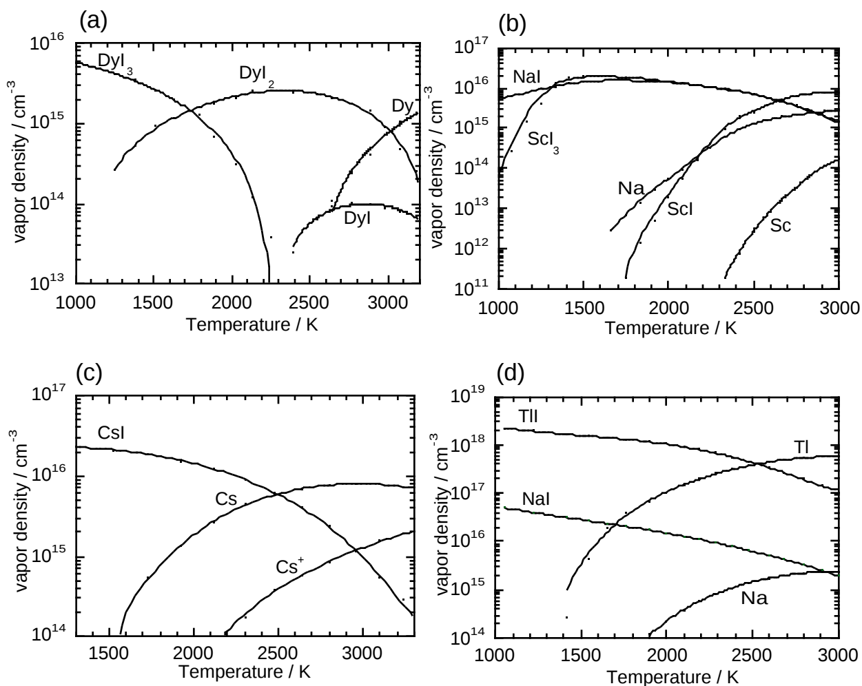
Figure 4.1 Relationship between the vapor densities of the various molecular and atomic species and temperature in (a) \text{DyI}_3/\text{Hg} , (b) \text{ScI}_3/\text{NaI}/\text{Hg} , (c) \text{CsI}/\text{Hg} , and (d) \text{TlI}/\text{NaI}/\text{Hg} arc discharge lamps in the literatures
