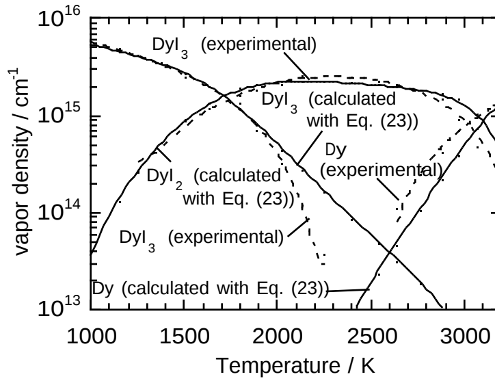
Figure 4.3 Vapor density of dysprosium metal and iodides in DyI 3 /Hg arc discharge lamps as a function of temperature. The solid and dashed lines denote those calculated with Eq. (4.23) and experimental ones, respectively.
