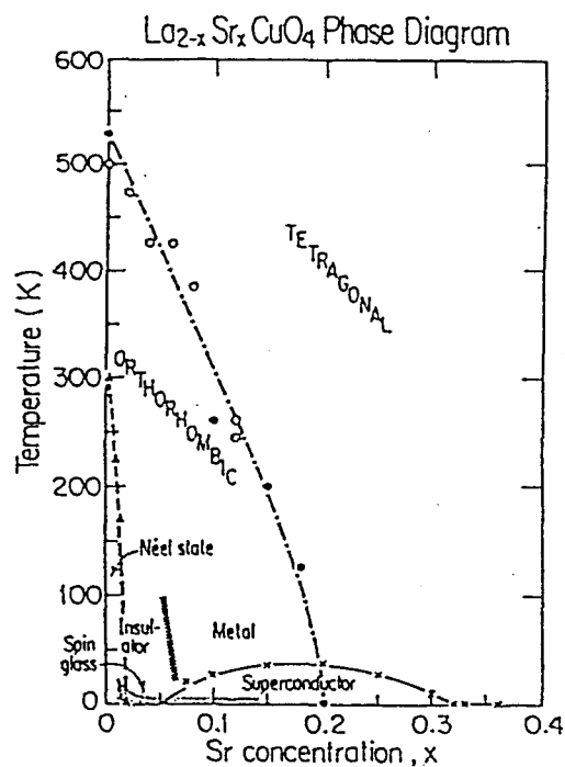
Fig.1-1-3. Phase diagram of \text{La}_{2-x}\text{Sr}_x\text{CuO}_4 . 3)
