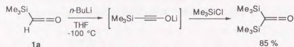
Scheme 13
