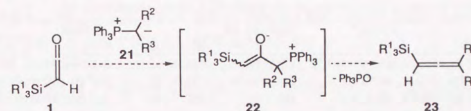
Scheme 16
