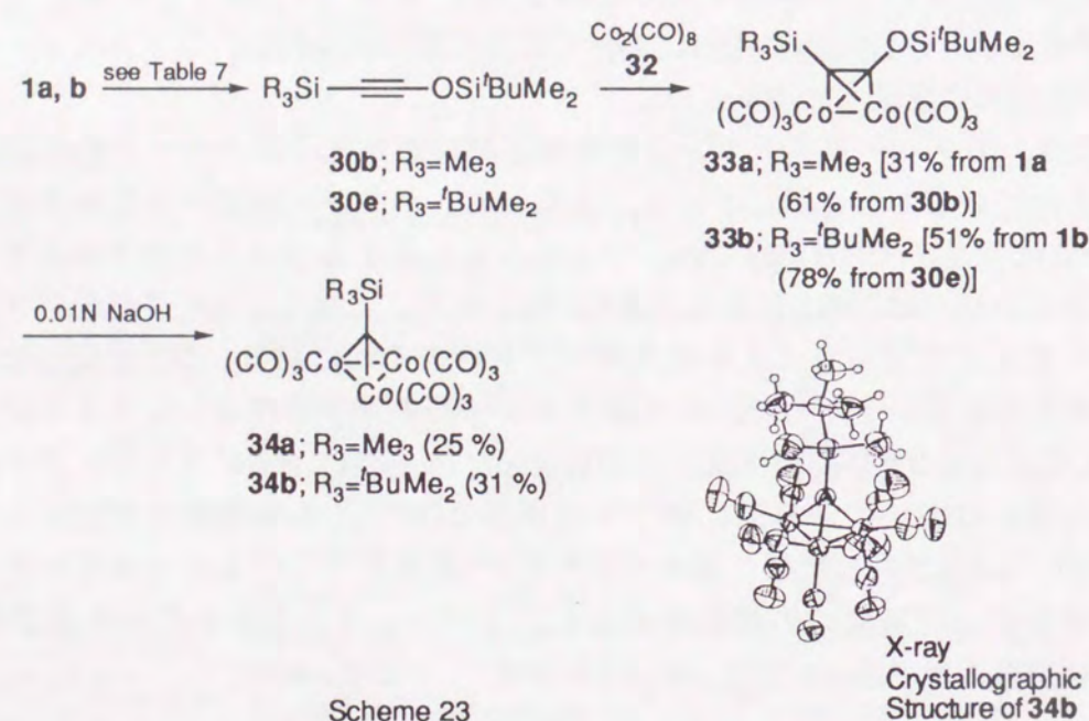
Scheme 23
