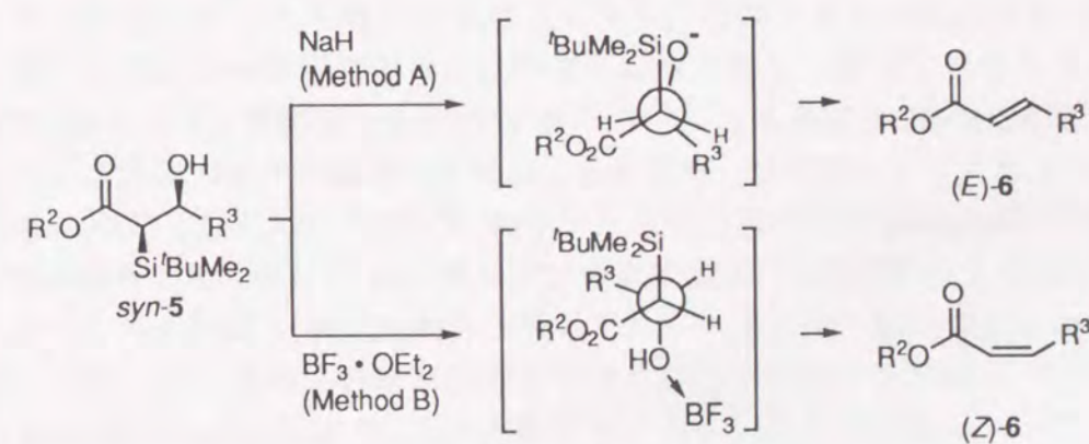
Scheme 5
