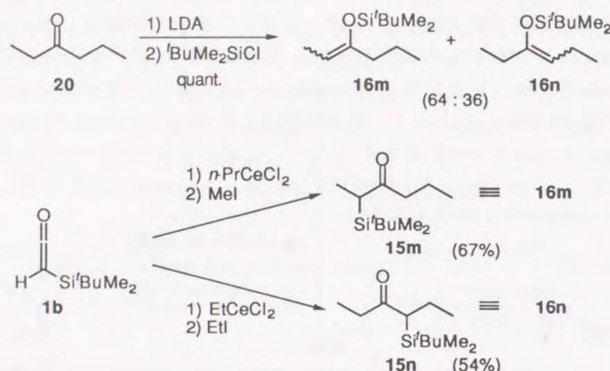
Scheme 15
