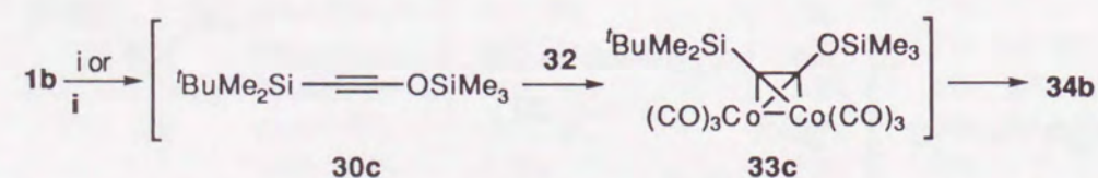
Scheme 24 Reagents: i, n BuLi then Me 3 SiCl, Co 2 (CO) 8 ( 32 ); ii, Me 3 SiOTf, Et 3 N, 32
